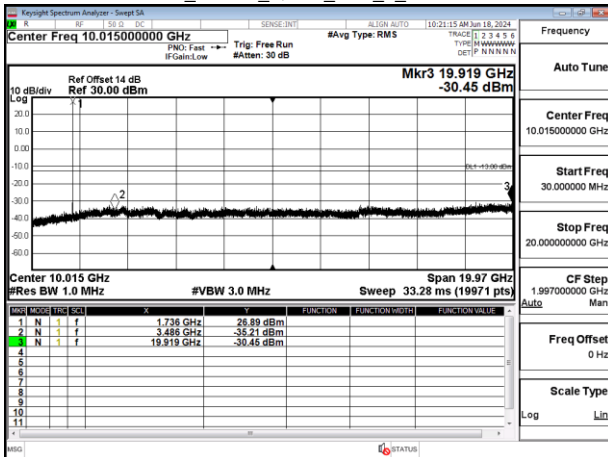
Band66_20MHz_QPSK_RB1_0_CH132322
