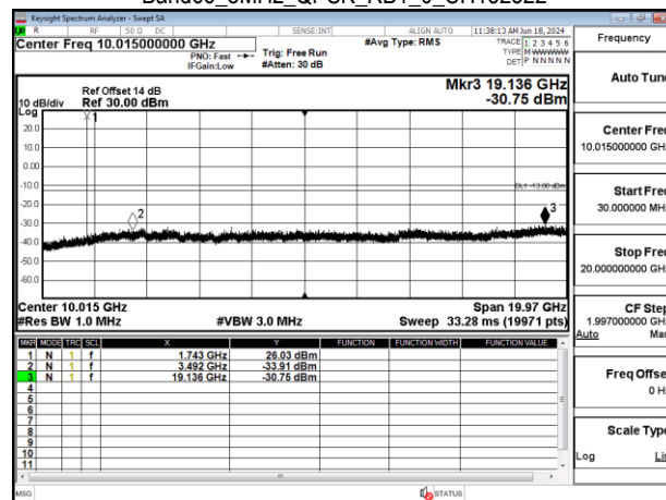
Band66 5MHz_QPSK_RB1_0_CH132322
