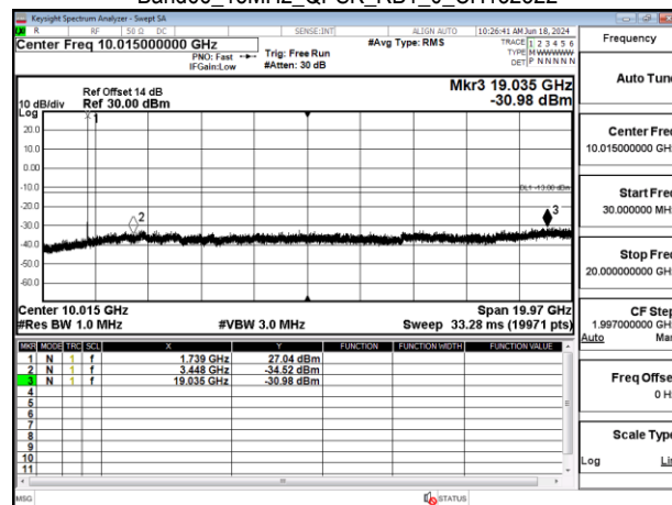
Band66_15MHz_QPSK_RB1_0_CH132322
