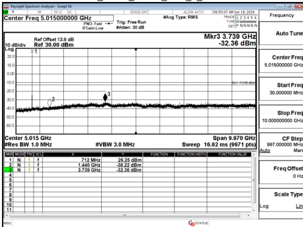
Band12_5MHz_QPSK_RB1_0_CH23155
