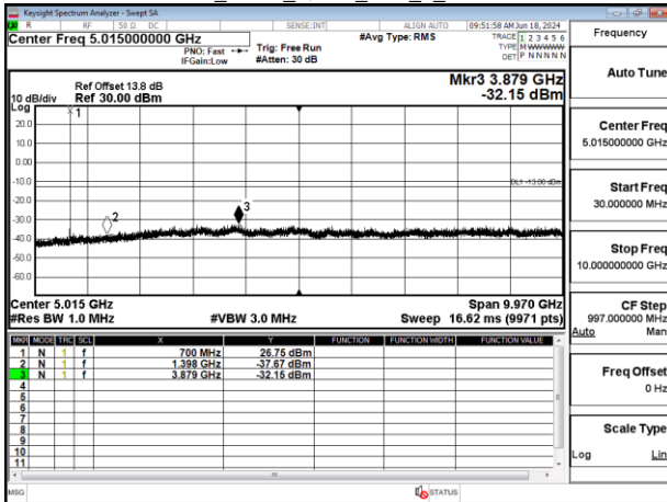
Band12_5MHz_QPSK_RB1_0_CH23095
