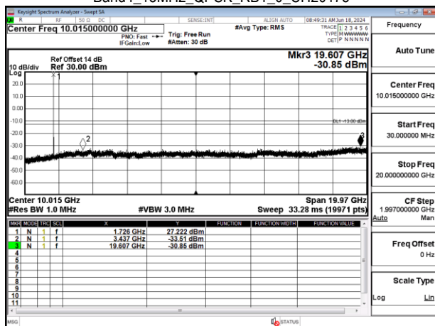
Band4_15MHz_QPSK_RB1_0_CH20325
