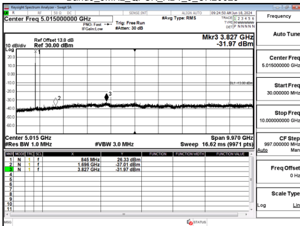
Band5_5MHz_QPSK_RB1_0_CH20625
