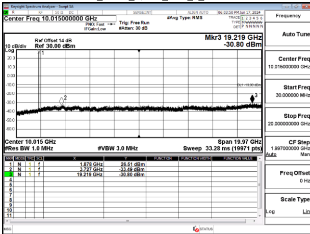
Band2_5MHz_QPSK_RB1_0_CH19175
