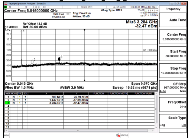
Band12_10MHz_QPSK_RB1_0_CH23095
