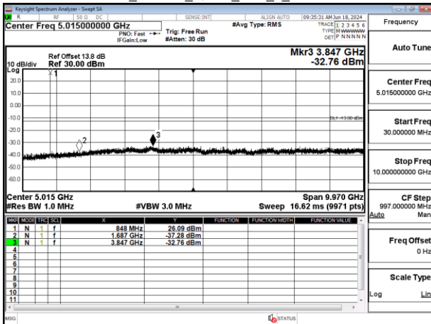
Band5_1.4MHz_QPSK_RB1_0_CH20643
