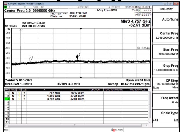
Band12_10MHz_QPSK_RB1_0_CH23130
