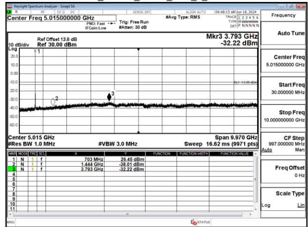
Band12_10MHz_QPSK_RB1_0_CH23130
