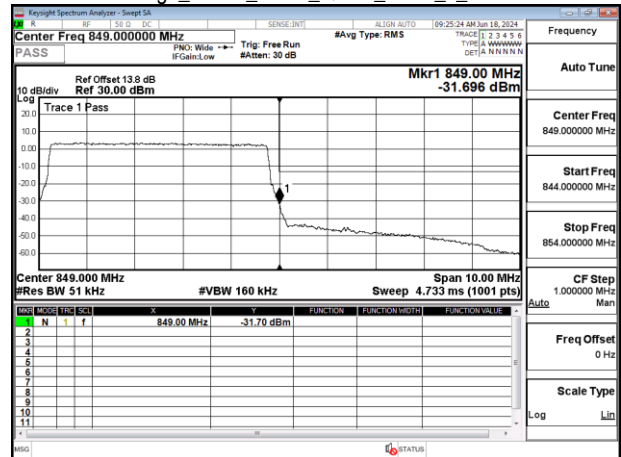
Band Edge_Band5_5MHz_QPSK_RB25_0_CH20625
