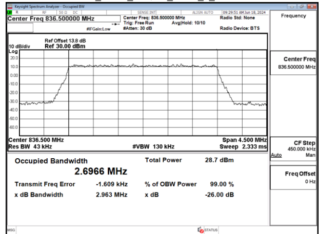
Band5_3MHz_64QAM_RB15_0_CH20635
