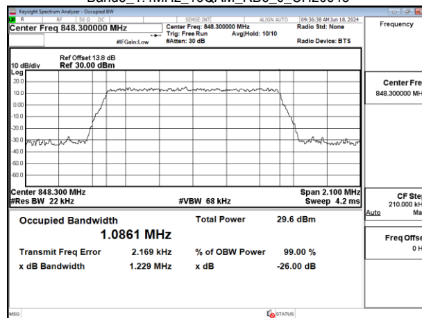
Band5_1.4MHz_16QAM_RB6_0_CH20643
