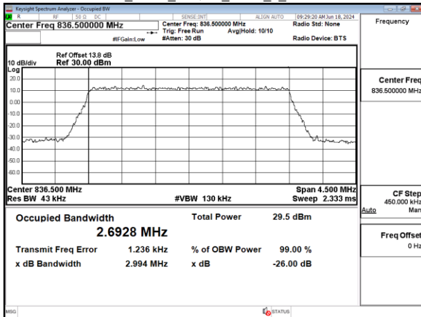
Band5_3MHz_16QAM_RB15_0_CH20635
