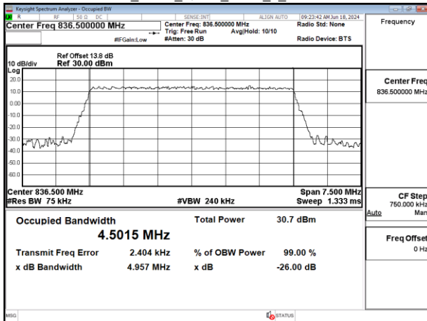
Band5_5MHz_QPSK_RB25_0_CH20625
