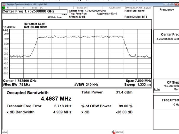
Band4_5MHz_QPSK_RB25_0_CH20375
