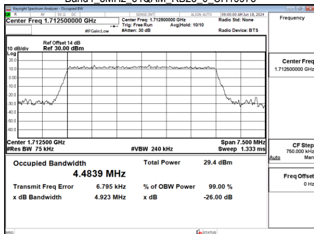
Band4_5MHz_64QAM_RB25_0_CH20175
