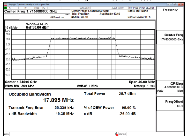
Band4_20MHz_64QAM_RB100_0_CH20300
