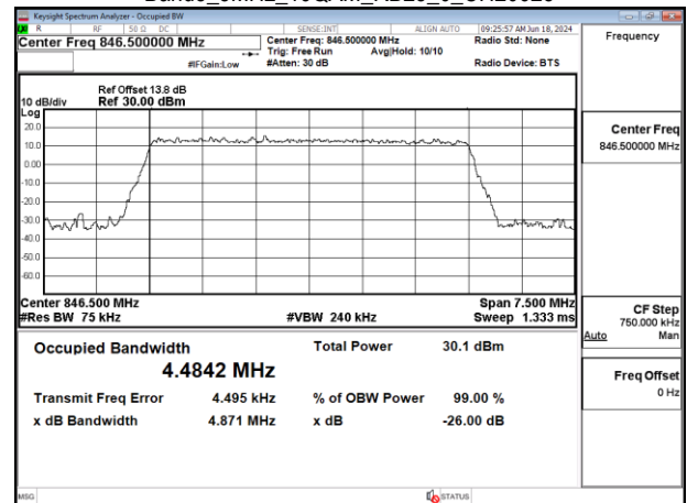
Band5_5MHz_16QAM_RB25_0_CH20625
