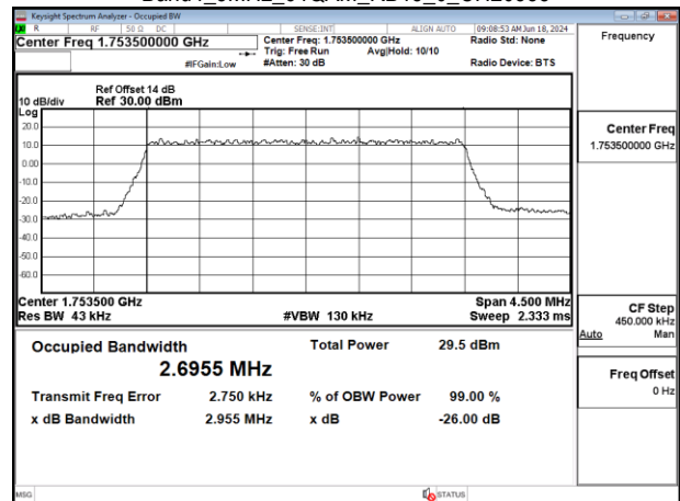
Band4_3MHz_64QAM_RB15_0_CH20385
