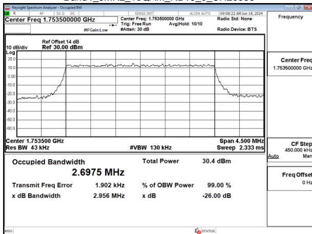
Band4_3MHz_16QAM_RB15_0_CH20385
