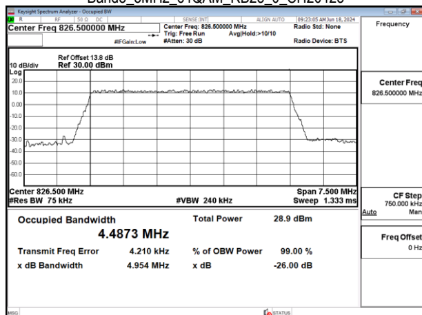
Band5_5MHz_64QAM_RB25_0_CH20525
