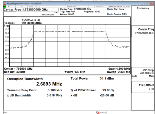
Band4_3MHz_QPSK_RB15_0_CH20385
