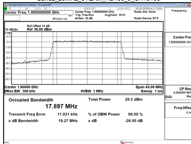
Band2 20MHz_64QAM_RB100_0_CH19100
