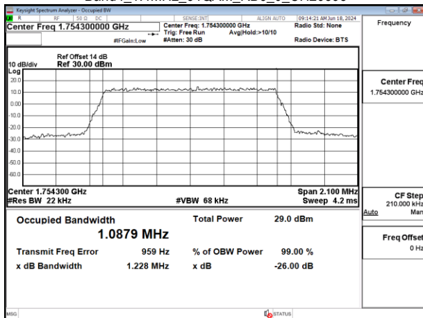
Band4_1.4MHz_64QAM_RB6_0_CH20393
