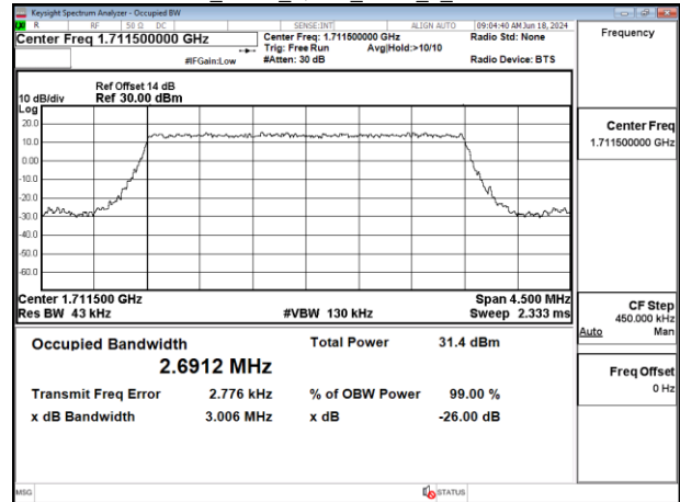
Band4_3MHz_QPSK_RB15_0_CH20175
