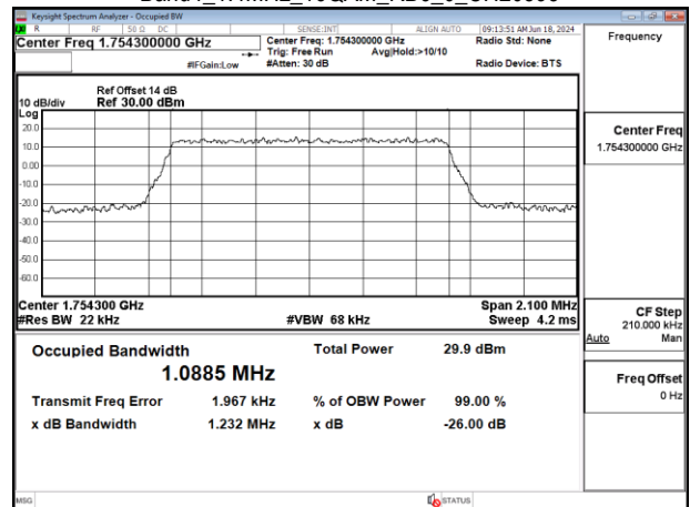
Band4_1.4MHz_16QAM_RB6_0_CH20393
