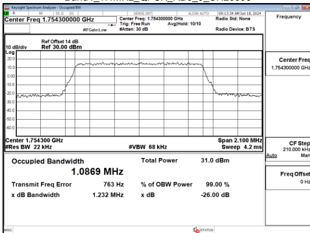
Band4_1.4MHz_QPSK_RB6_0_CH20393
