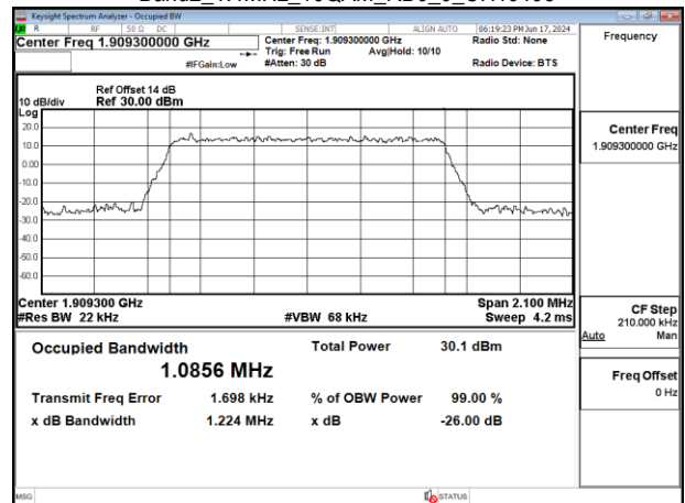
Band2_1.4MHz_16QAM_RB6_0_CH19193
