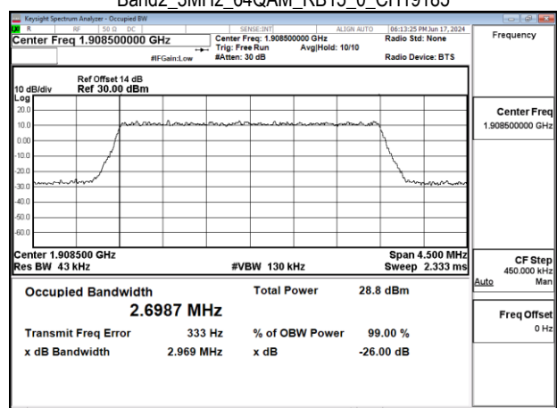
Band2_3MHz_64QAM_RB15_0_CH19185
