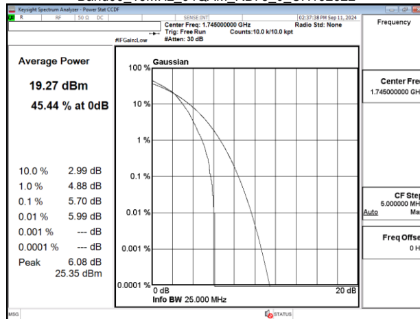
Band66_15MHz_64QAM_RB75_0_CH132322
