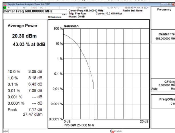
Band71_20MHz_64QAM_RB100_0_CH133372
