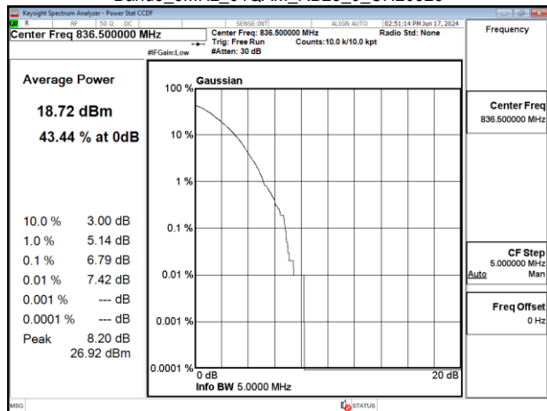
Band5_5MHz_64QAM_RB25_0_CH20625
