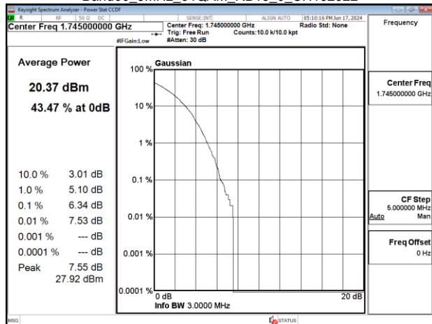
Band66_3MHz_64QAM_RB15_0_CH132322
