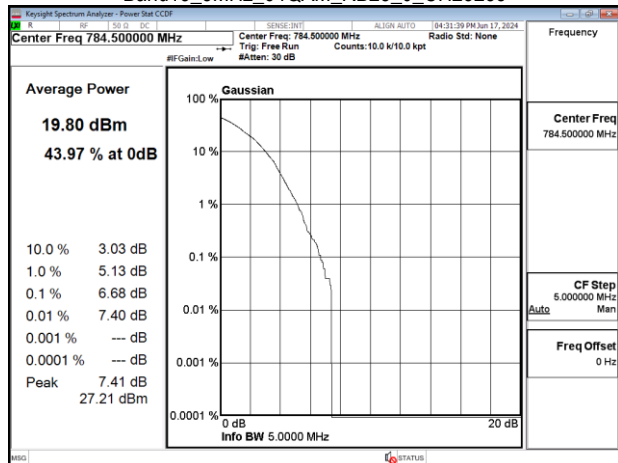
Band13_5MHz_64QAM_RB25_0_CH23255
