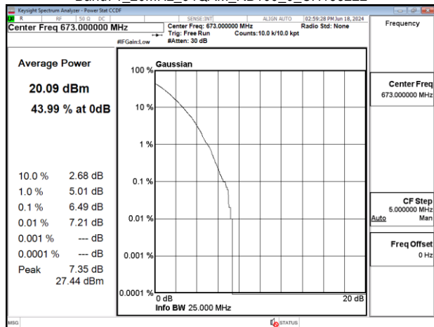
Band71_20MHz_64QAM_RB100_0_CH133222
