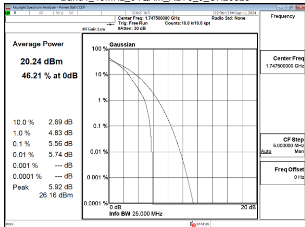
Band4_15MHz_64QAM_RB75_0_CH20325
