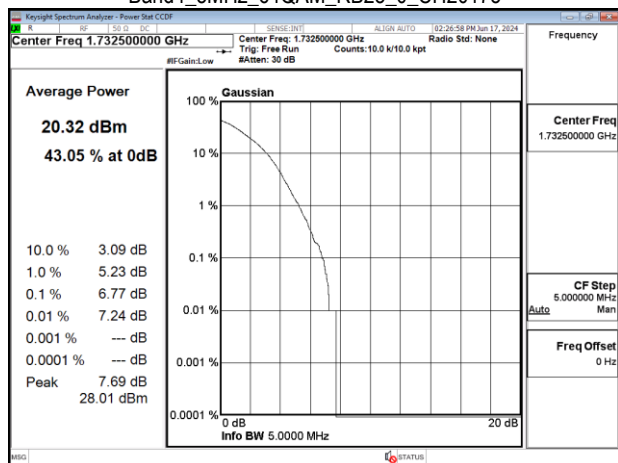
Band4_5MHz_64QAM_RB25_0_CH20375
