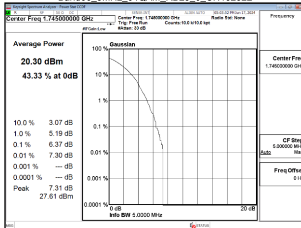
Band66_5MHz_64QAM_RB25_0_CH132322
