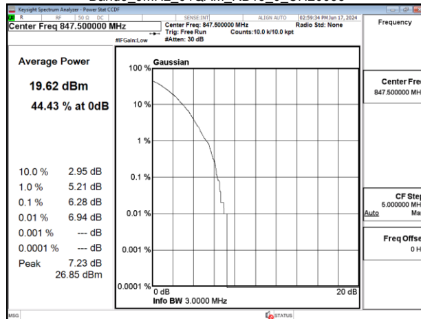
Band5_3MHz_64QAM_RB15_0_CH20635
