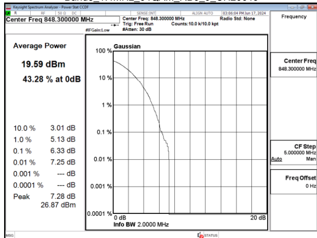
Band5_1.4MHz_64QAM_RB6_0_CH20643
