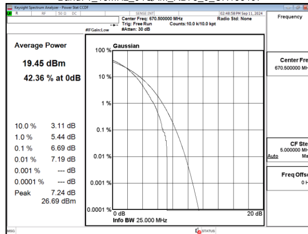
Band71_15MHz_64QAM_RB75_0_CH133297
