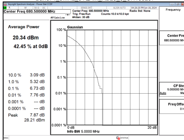
Band71 5MHz 64QAM_RB25_0_CH133297
