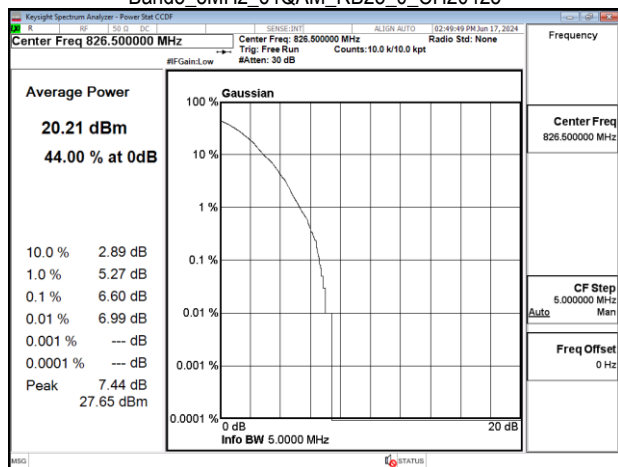
Band5_5MHz_64QAM_RB25_0_CH20525
