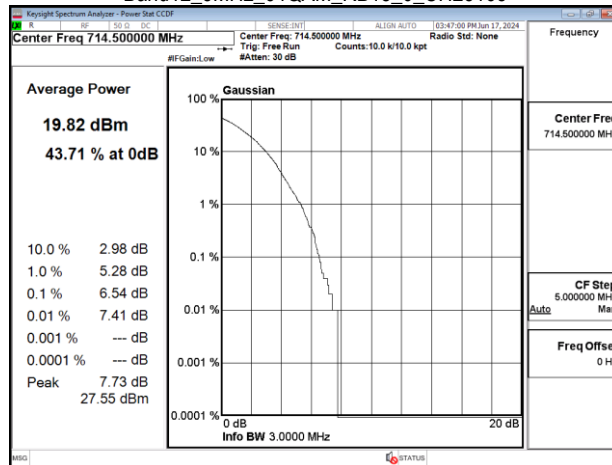
Band12 3MHz 64QAM_RB15_0_CH23165
