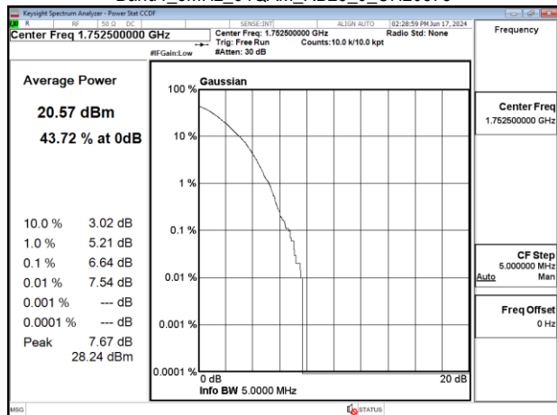
Band4_5MHz_64QAM_RB25_0_CH20375
