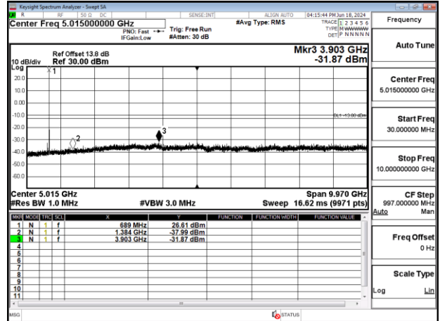
Band71_15MHz_QPSK_RB1_0_CH133197
