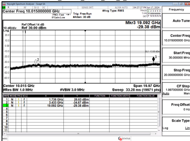
Band66_20MHz_QPSK_RB1_0_CH132322
