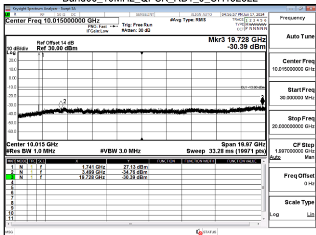
Band66_10MHz_QPSK_RB1_0_CH132322
