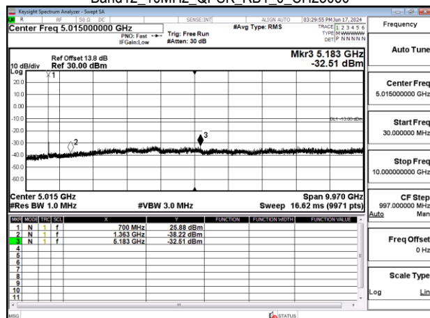
Band12_10MHz_QPSK_RB1_0_CH23095
