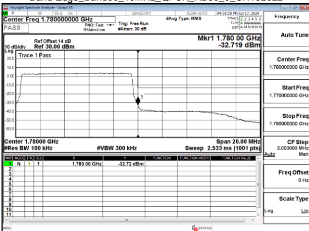
Band Edge_Band66_10MHz_QPSK_RB50_0_CH132622
