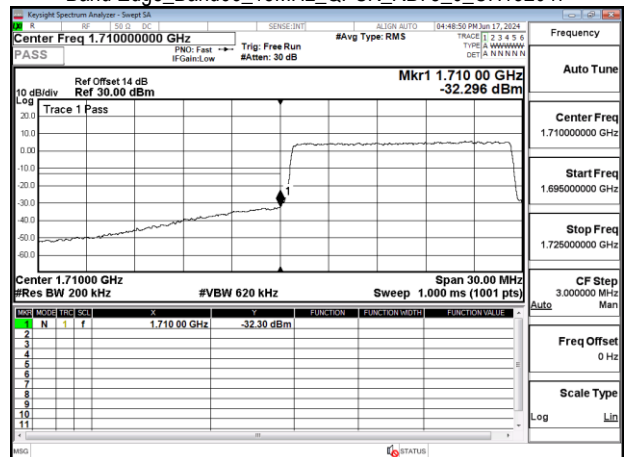
Band Edge_Band66_15MHz_QPSK_RB75_0_CH132047
