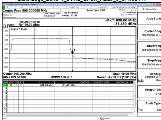
Band Edge_Band71_5MHz_QPSK_RB25_0_CH133447
