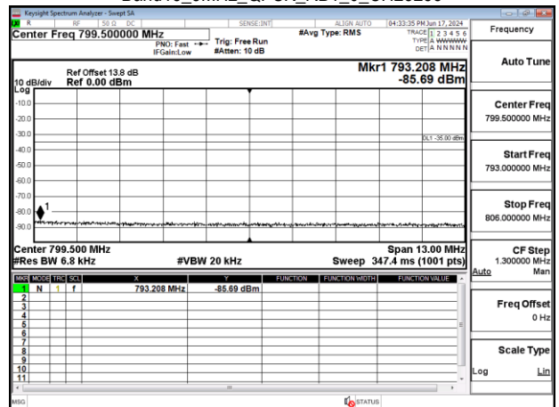
Band13 5MHz_QPSK_RB1_0_CH23255
