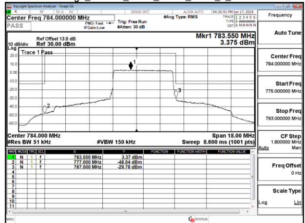
Band Edge_Band13_5MHz_QPSK_RB25_0_CH23255
