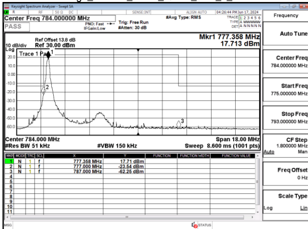
Band Edge_Band13_5MHz_QPSK_RB1_0_CH23205
