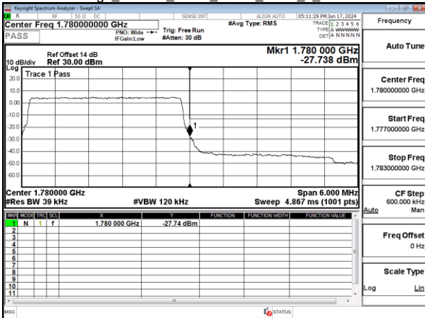
Band Edge_Band66_5MHz_QPSK_RB1_0_CH131997
