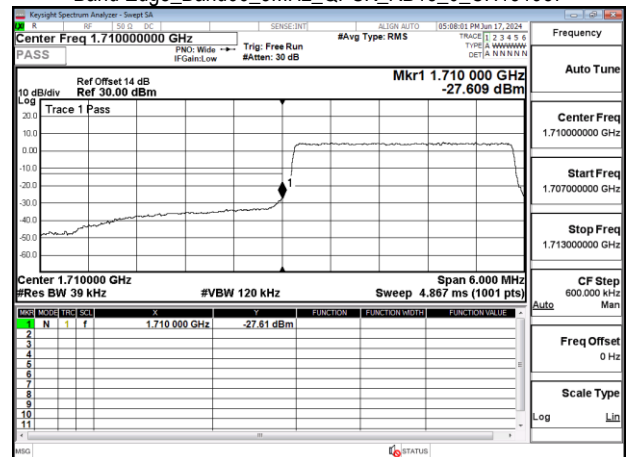
Band Edge_Band66_3MHz_QPSK_RB15_0_CH131987
