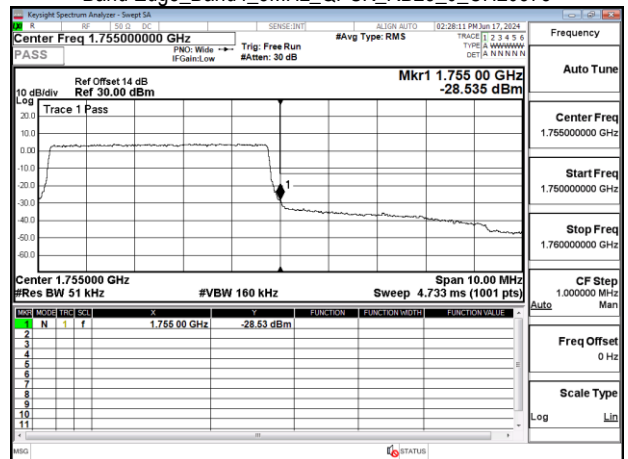
Band Edge_Band4_5MHz_QPSK_RB25_0_CH20375
