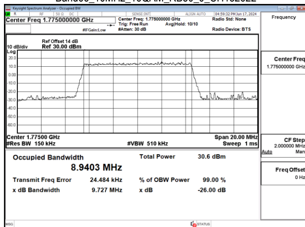
Band66_10MHz_16QAM_RB50_0_CH132622
