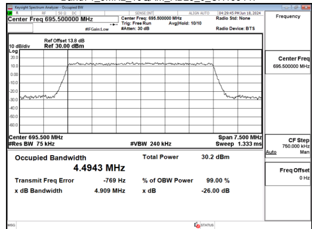
Band71_5MHz_16QAM_RB25_0_CH133447
