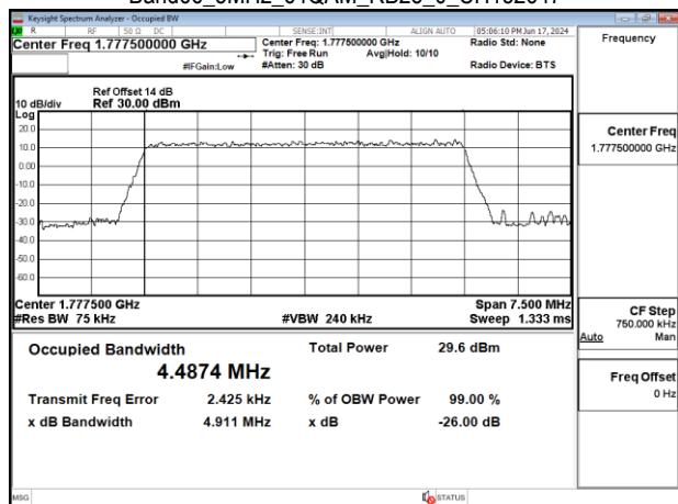
Band66_5MHz_64QAM_RB25_0_CH132647
