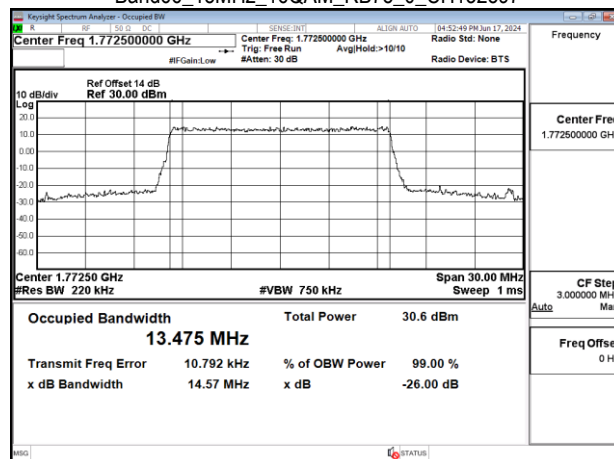
Band66_15MHz_16QAM_RB75_0_CH132597
