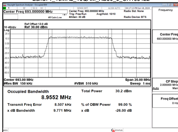
Band71_10MHz_16QAM_RB50_0_CH133422
