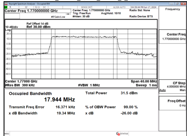
Band66_20MHz_QPSK_RB100_0_CH132572
