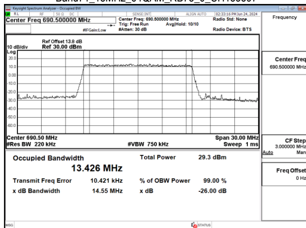
Band71_15MHz_64QAM_RB75_0_CH133397
