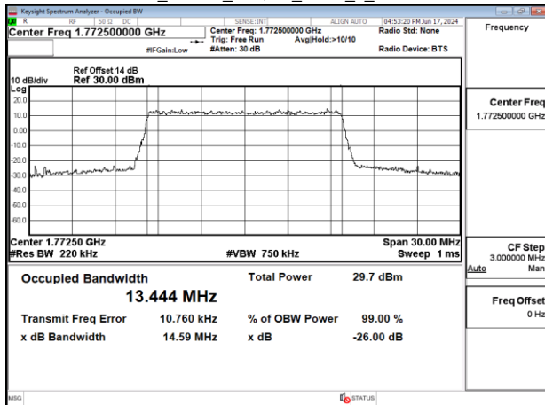
Band66_15MHz_64QAM_RB75_0_CH132597
