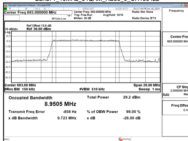
Band71_10MHz_64QAM_RB50_0_CH133422
