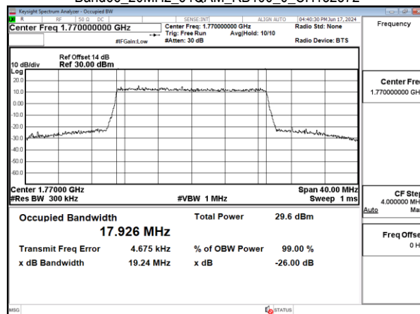
Band66 20MHz_64QAM_RB100_0_CH132572
