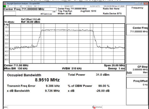
Band12_10MHz_QPSK_RB50_0_CH23130
