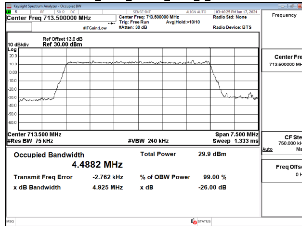
Band12_5MHz_16QAM_RB25_0_CH23155
