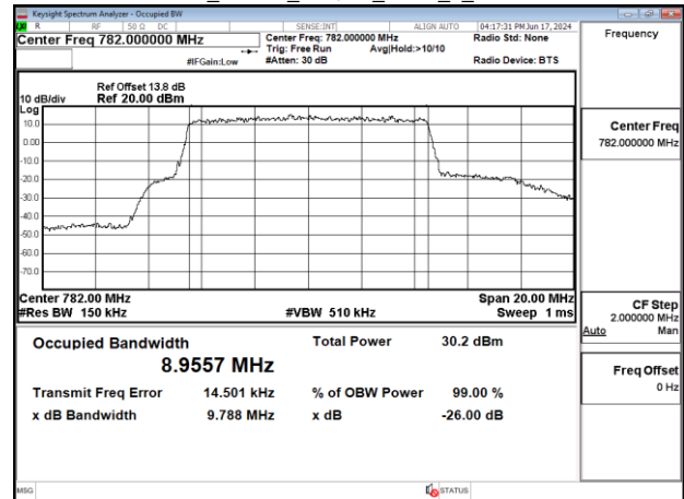
Band13_10MHz_64QAM_RB50_0_CH23230
