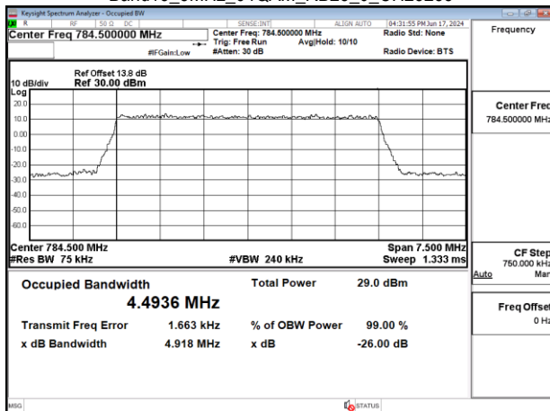
Band13_5MHz_64QAM_RB25_0_CH23255
