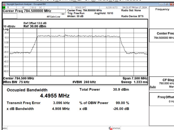
Band13_5MHz_QPSK_RB25_0_CH23255
