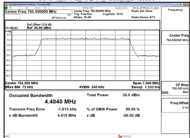
Band13_5MHz_16QAM_RB25_0_CH23255
