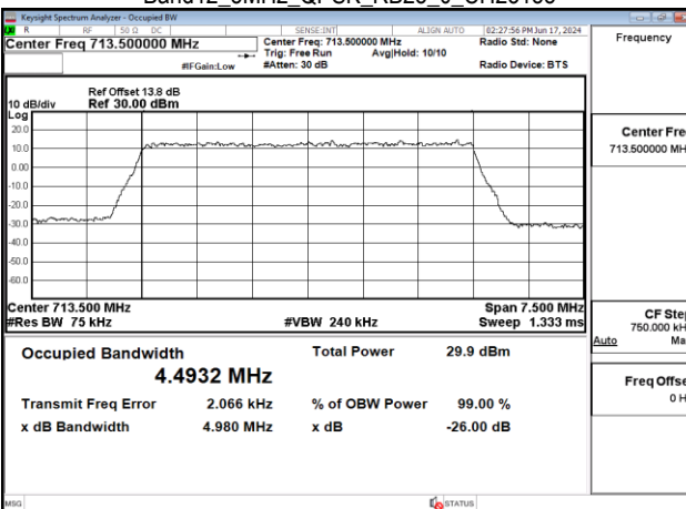
Band12_5MHz_QPSK_RB25_0_CH23155
