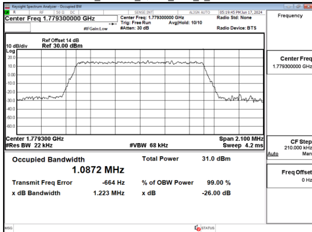
Band66_1.4MHz_QPSK_RB6_0_CH132665
