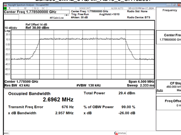
Band66_3MHz_64QAM_RB15_0_CH132657
