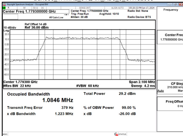
Band66_1.4MHz_64QAM_RB6_0_CH132665
