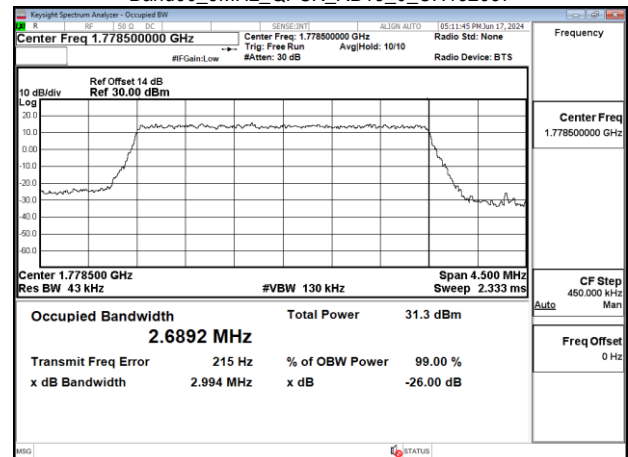
Band66_3MHz_QPSK_RB15_0_CH132657
