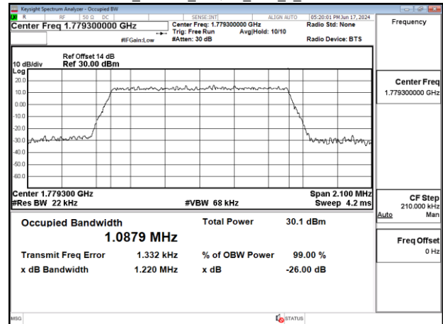
Band66_1.4MHz_16QAM_RB6_0_CH132665
