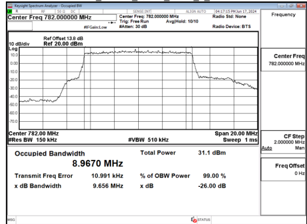
Band13_10MHz_16QAM_RB50_0_CH23230
