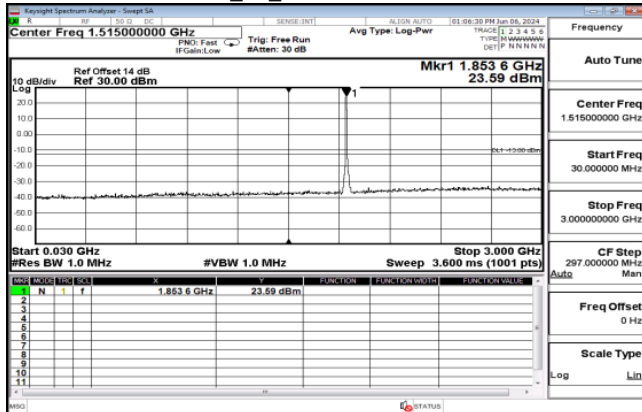
HSUPA_B2_LowCH9262-1852.4
