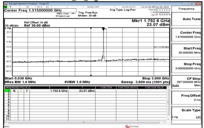
HSUPA_B4_HighCH1513-1752.6
