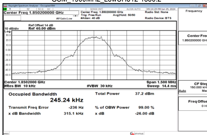
GSM_1900MHz_LowCH512-1850.2
