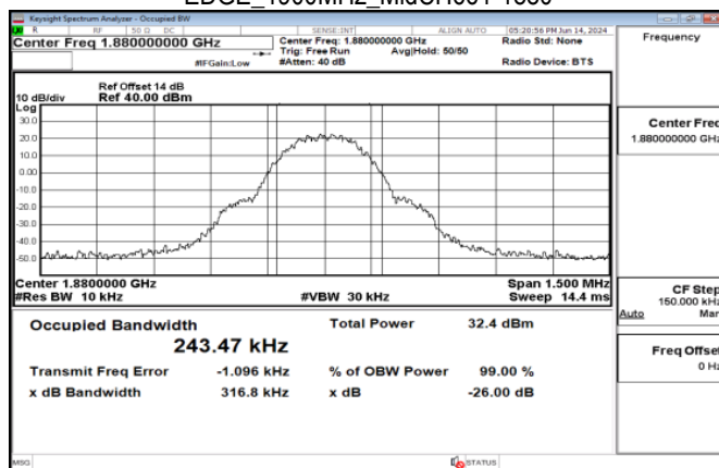
EDGE_1900MHz_MidCH661-1880
