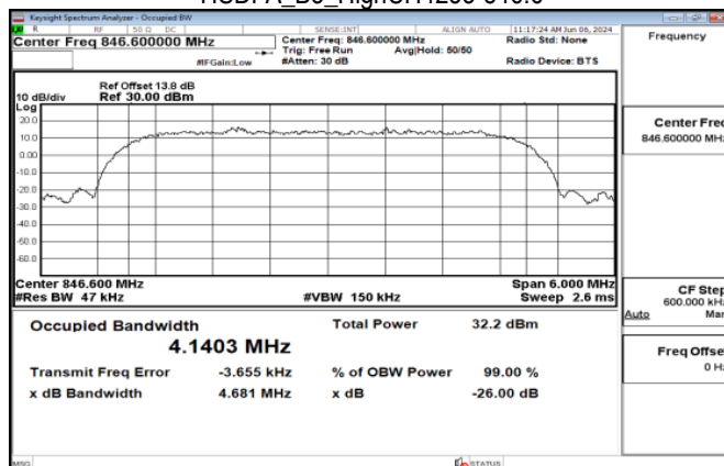
HSDPA_B5_HighCH4233-846.6
