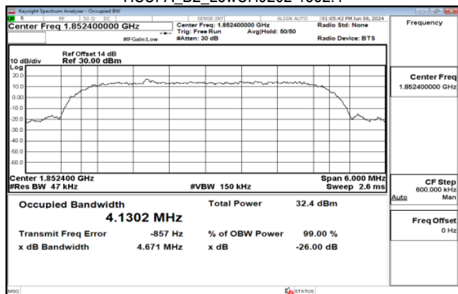
HSUPA_B2_LowCH9262-1852.4
