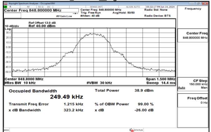
GPRS_850MHz_HighCH251-848.8
