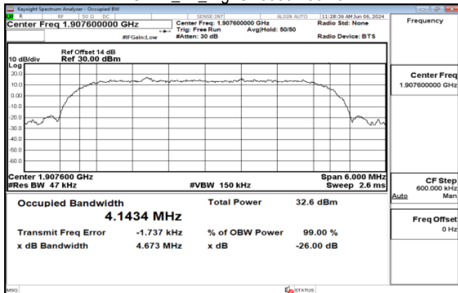
HSDPA_B2_HighCH9538-1907.6
