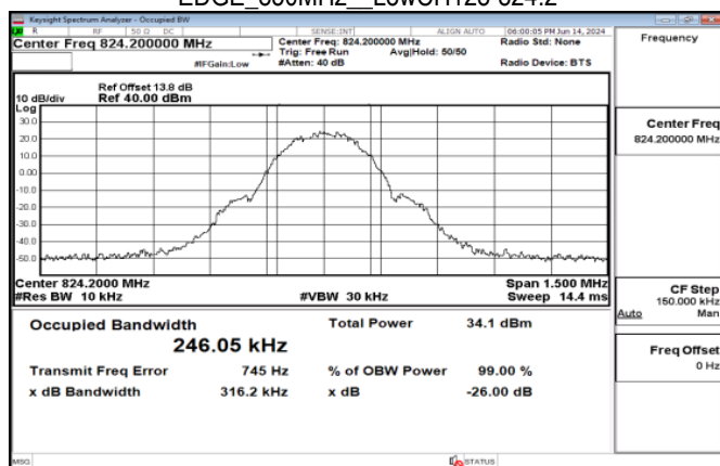
EDGE_850MHz_LowCH128-824.2
