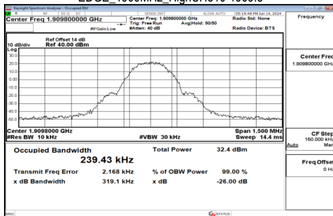
EDGE_1900MHz_HighCH810-1909.8
