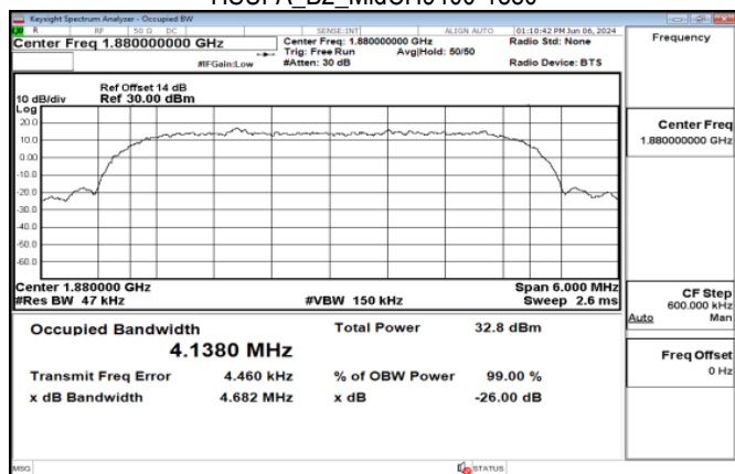
HSUPA_B2_MidCH9400-1880
