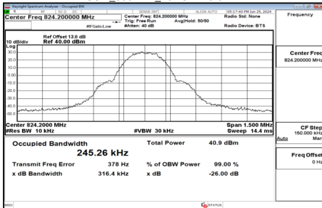
GSM_850MHz_LowCH128-824.2
