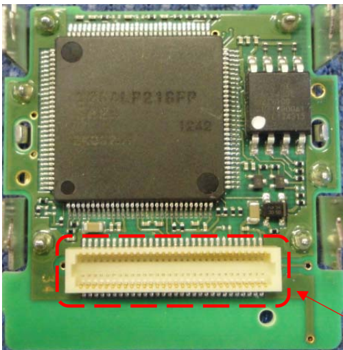
Bottom side view
