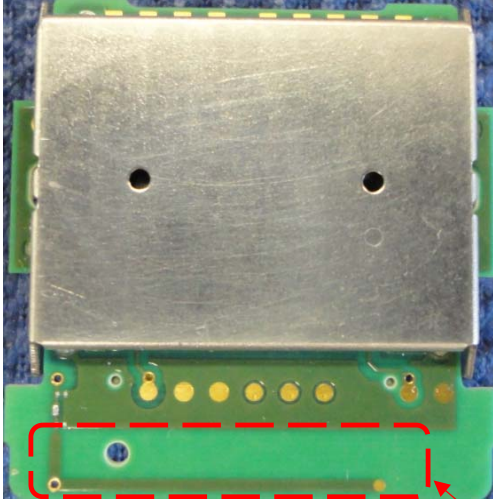
Shield cover side view
