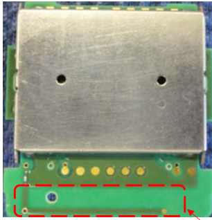
Shield cover side view
