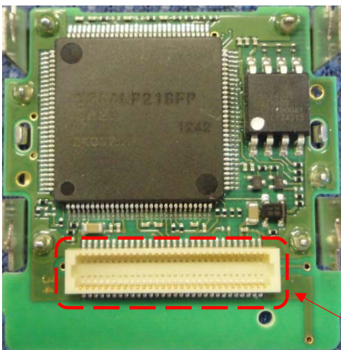
Bottom side view
