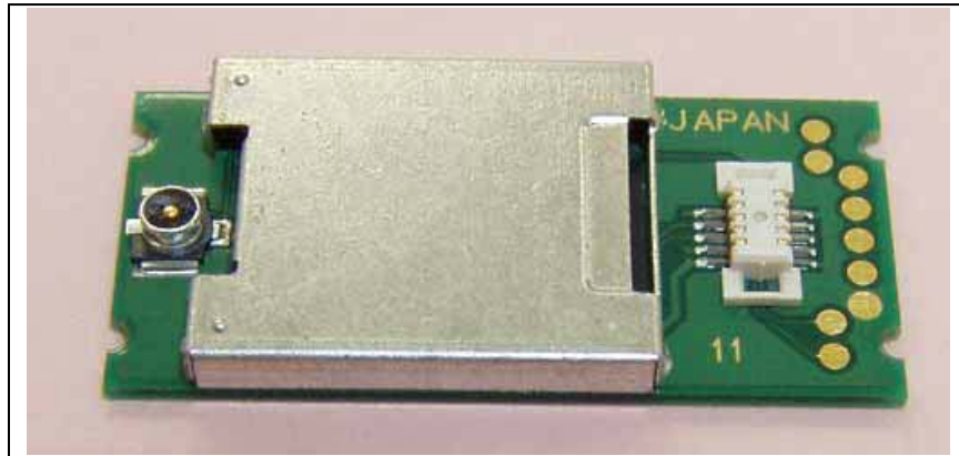
Top with shield cover
