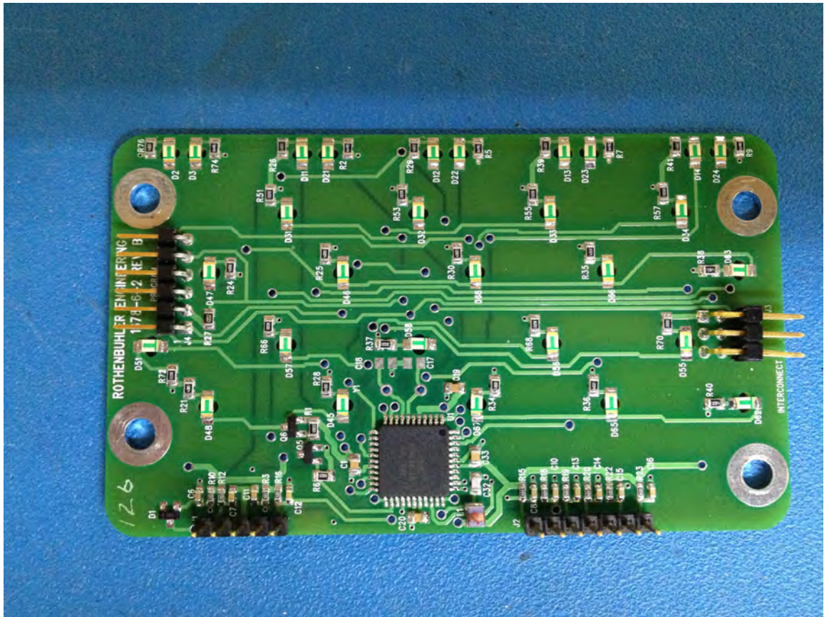
LED PCBA – Bottom
