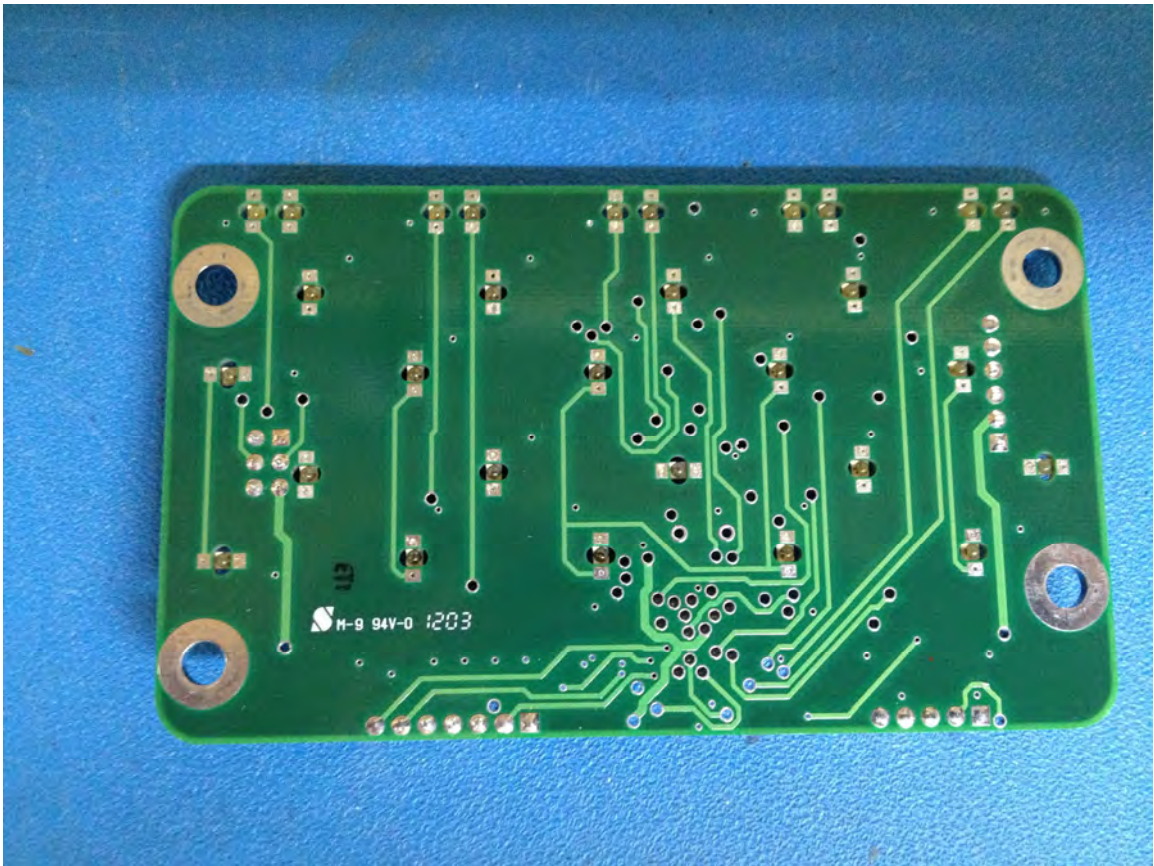
LED PCBA – Top
