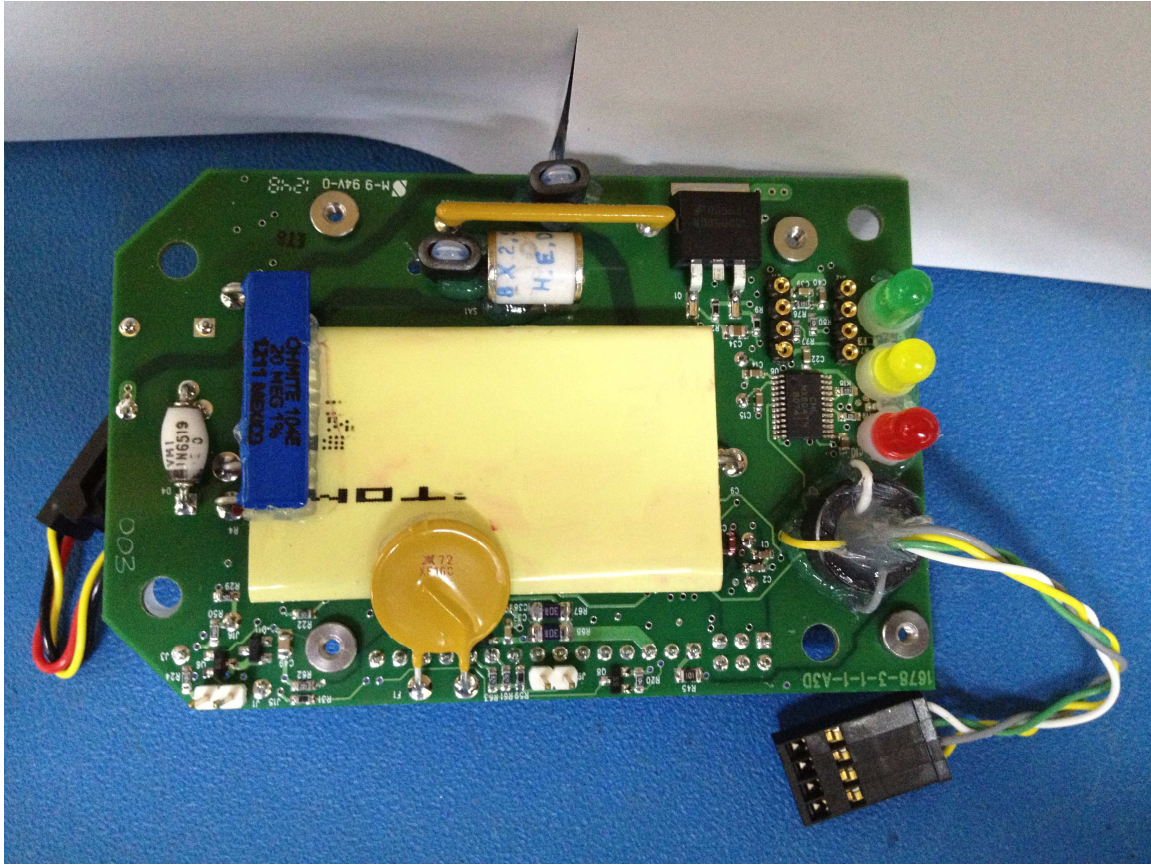
Microcontroller PCBA – Bottom
