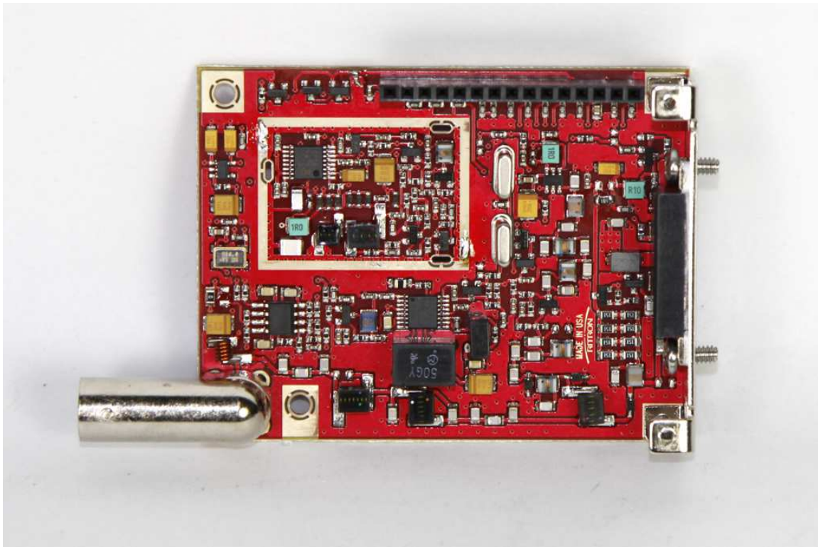
RF Transceiver Board – Shield Removed (Optional BNC connector shown instead of MMCX Cable)
