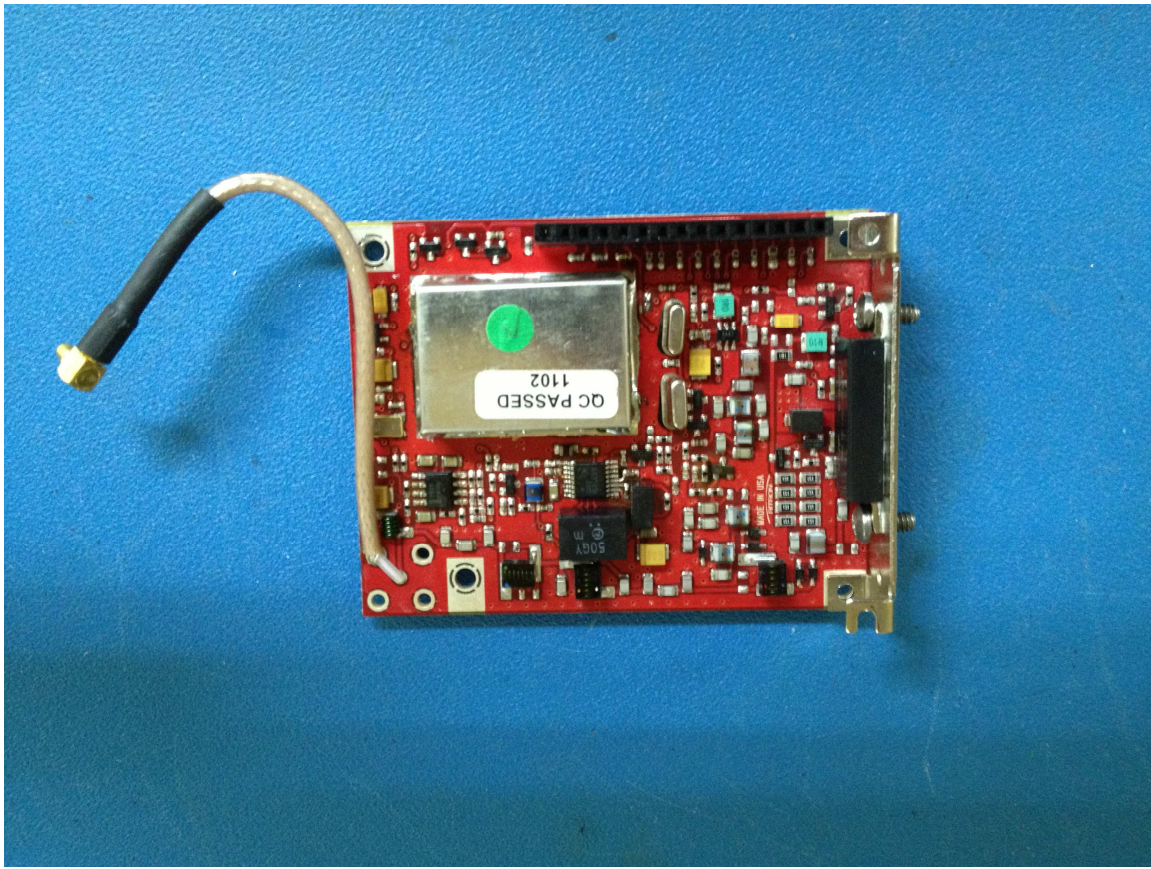
RF Transceiver Board – Top
