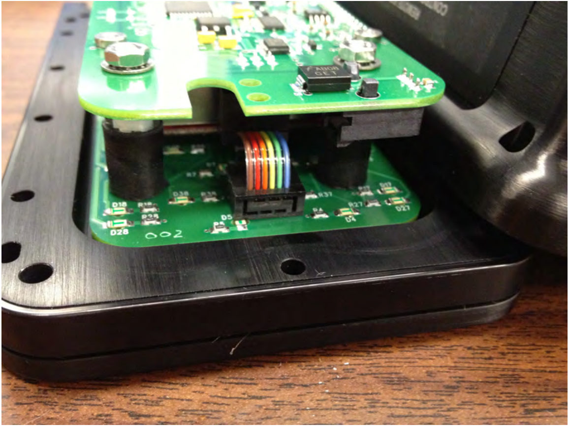
Electronics Assembly – Bottom End View
