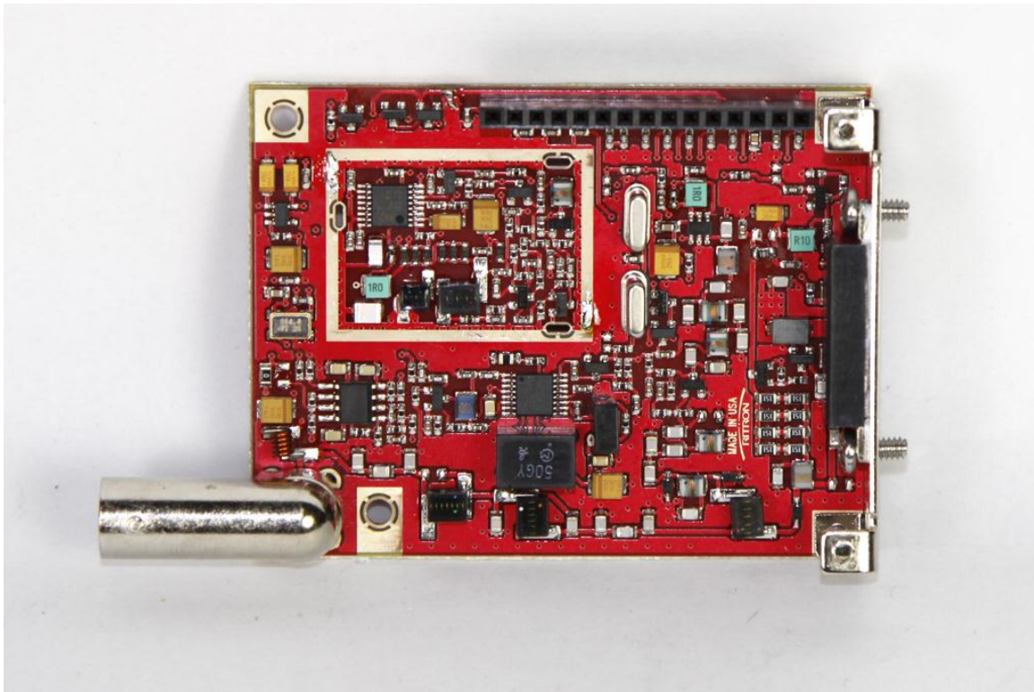
RF Transceiver Board – Shield Removed
