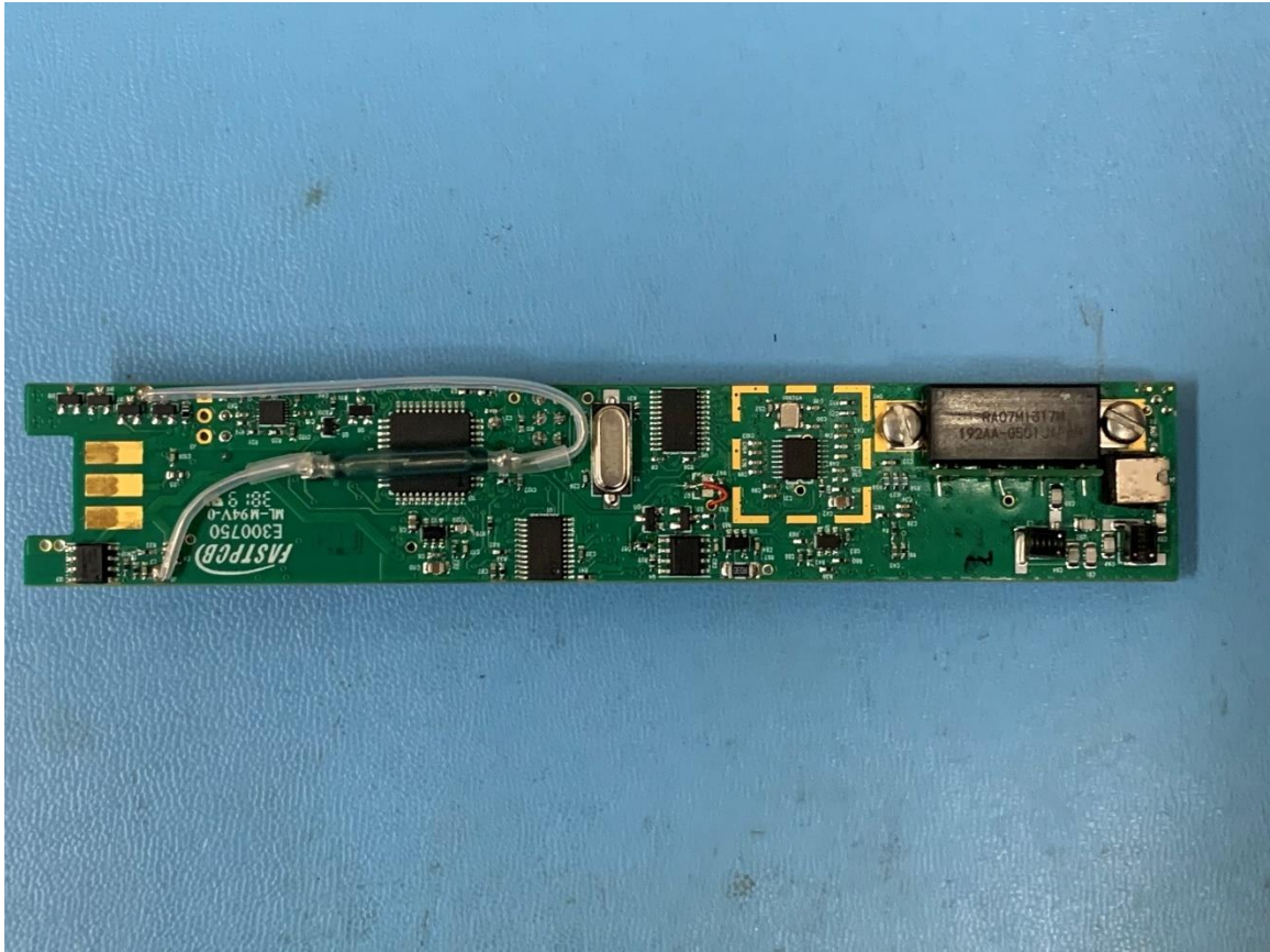
Figure 3 Main PCB Bottom Side
