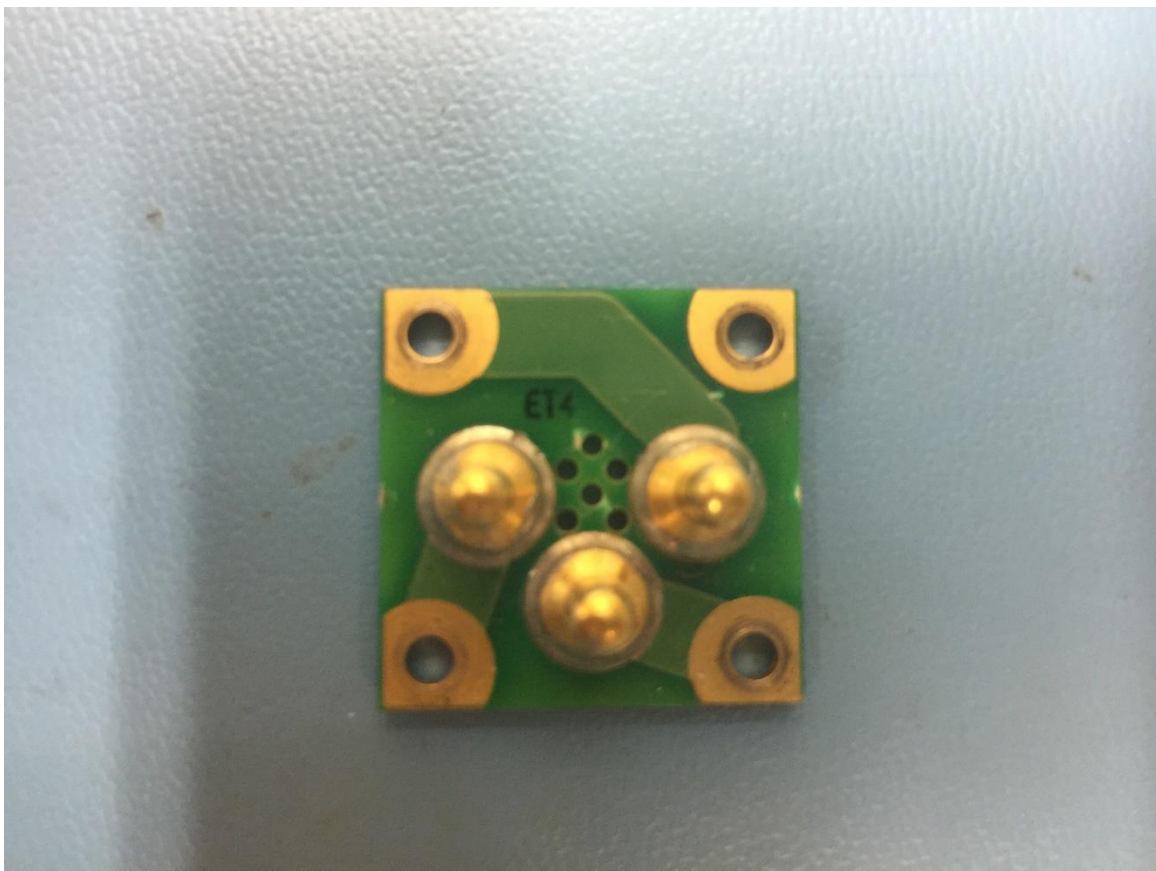
Figure 8 Charge PCB Front
