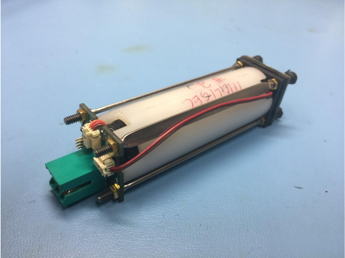
Figure 5 Battery Assembly
