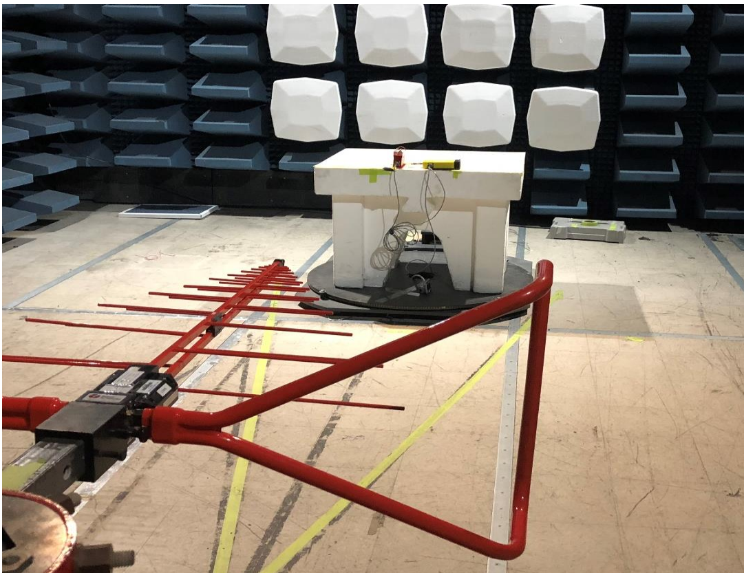
Radiated Emissions 3m SAC Setup – Photo2
