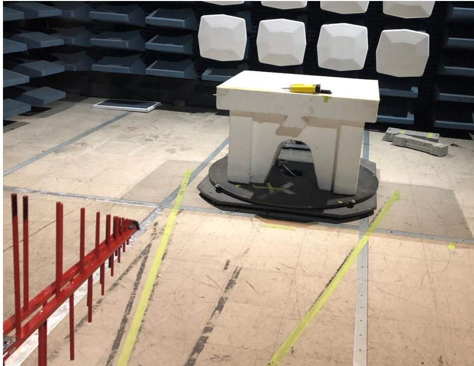
Radiated Emissions 3m SAC Setup – Photo1
