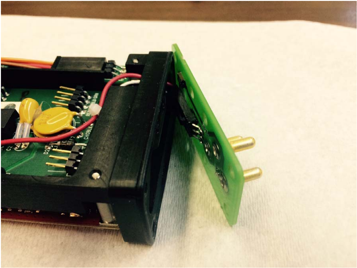
Picture 10 1100-5-2 Internal Assembly Interface Board Connections
