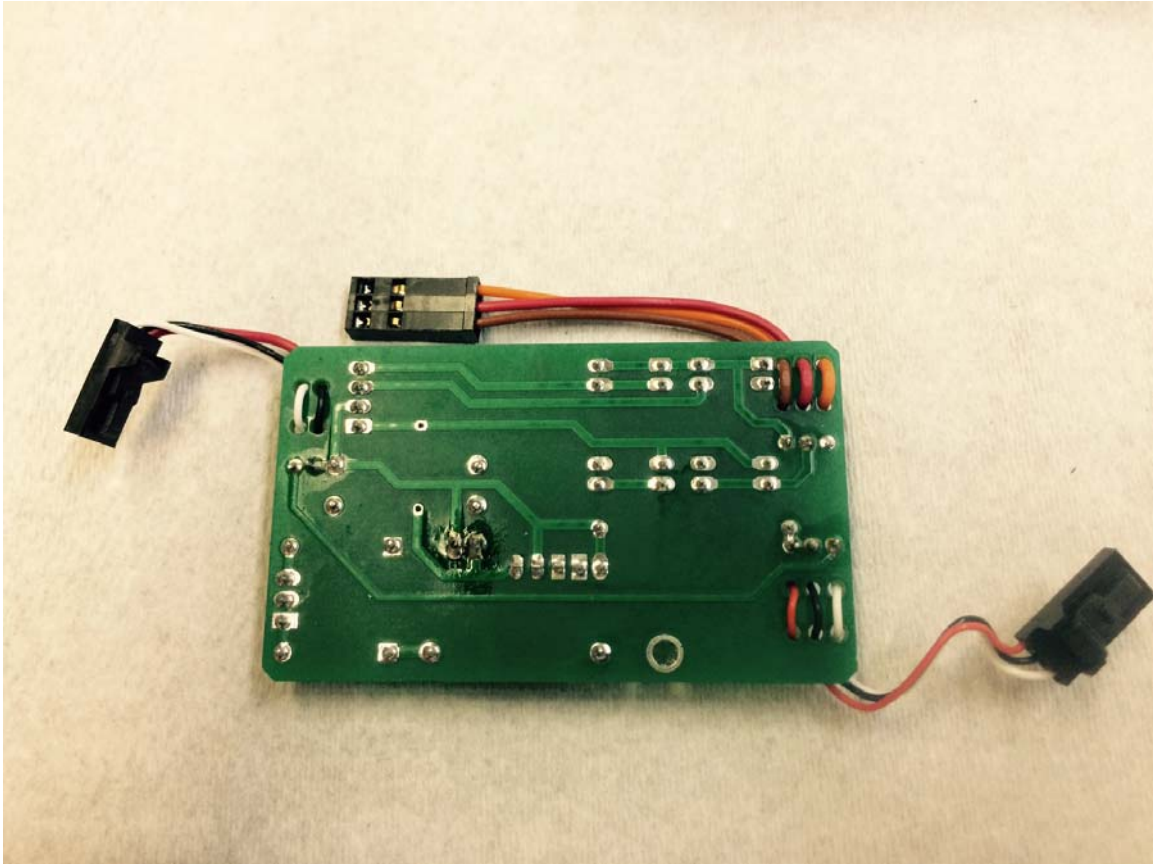
Picture 12 1100-5-2-1 Voltage Regulator Board Bottom View
