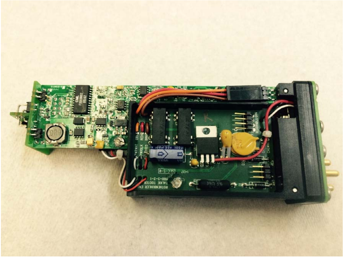
Picture 5 1100-5-2 Internal Assembly Top View
