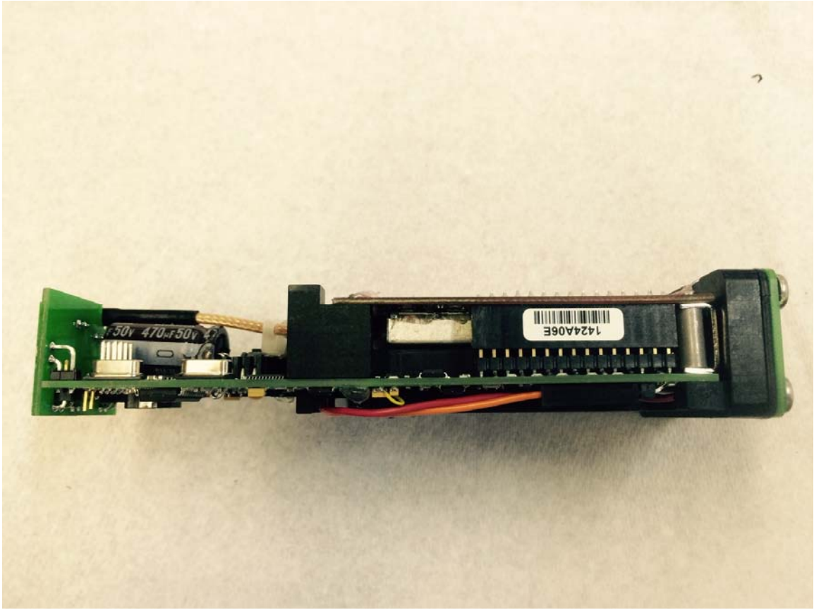
Picture 7 1100-5-2 Internal Assembly Side View
