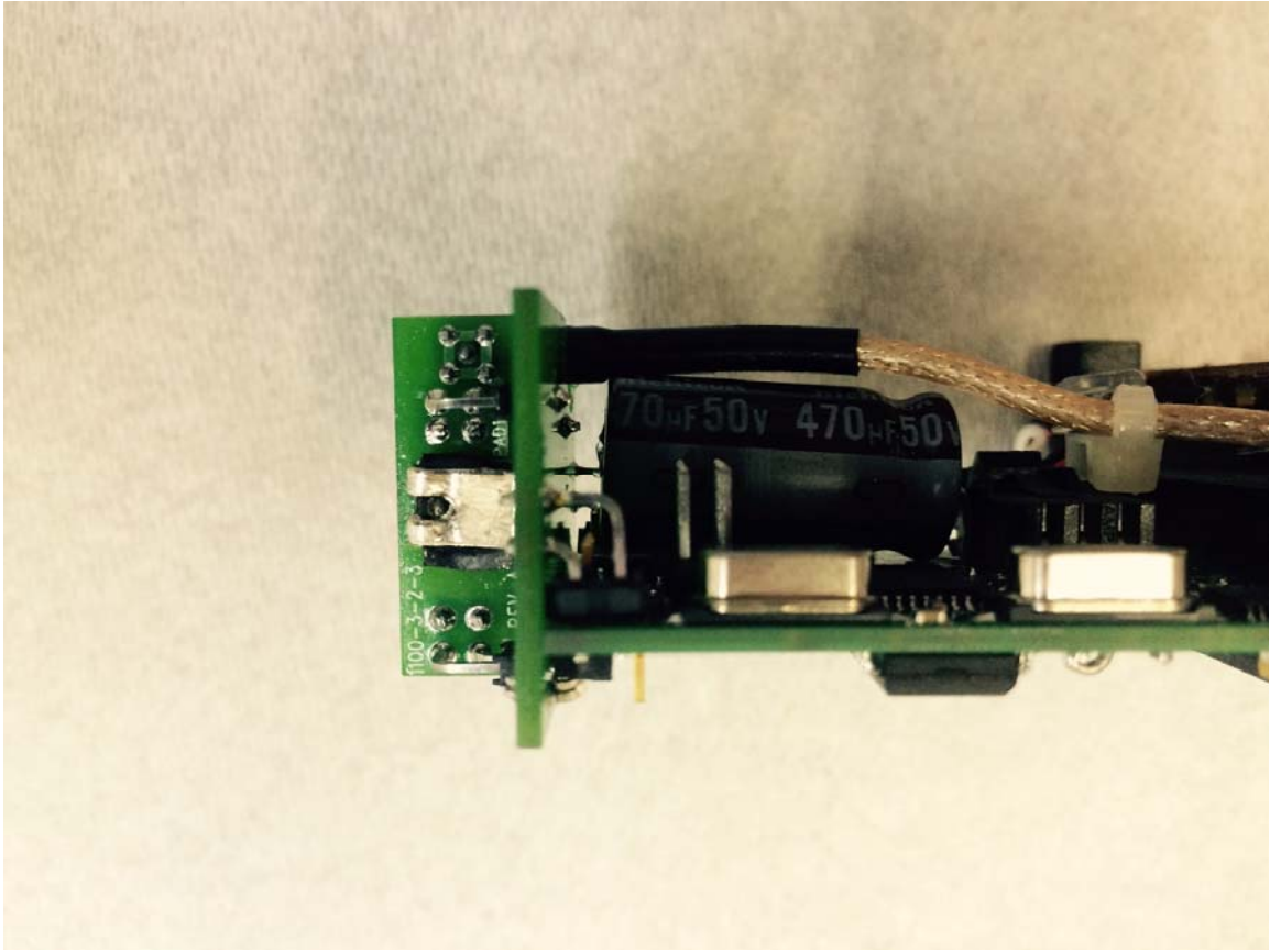
Picture 7 1100-3-2 Internal Assembly Antenna Interface Top View
