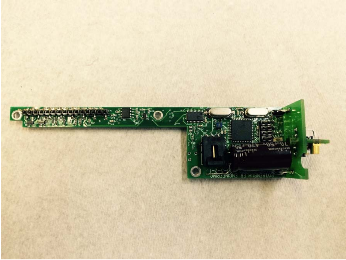
Picture 2 1100-3-2 Digital Board Bottom View
