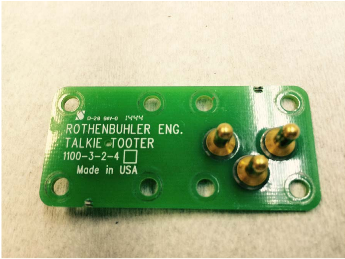
Picture 14 1100-3-2-4 Charge Interface Board Top View
