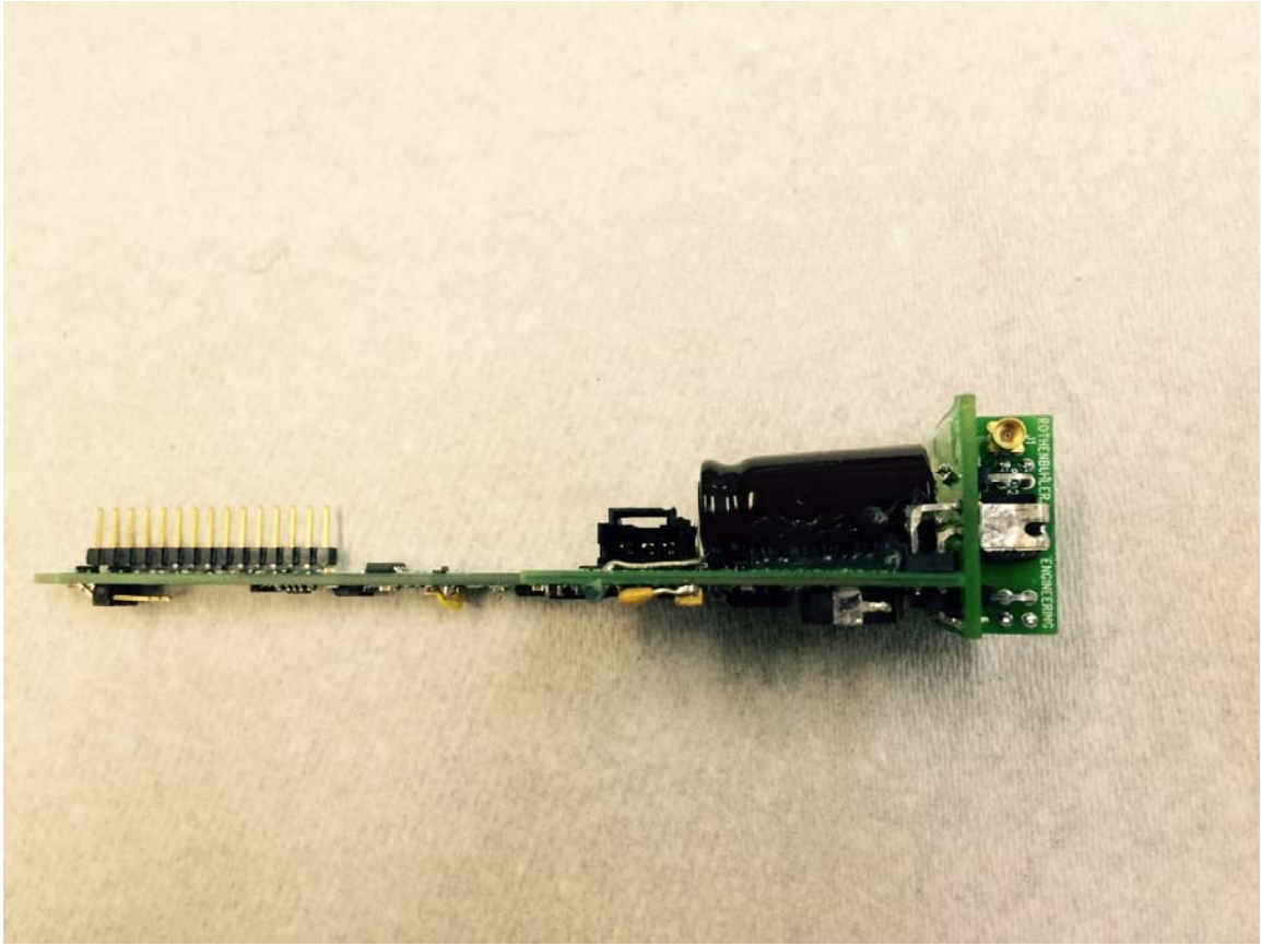
Picture 4 1100-3-2 Digital Board Side View
