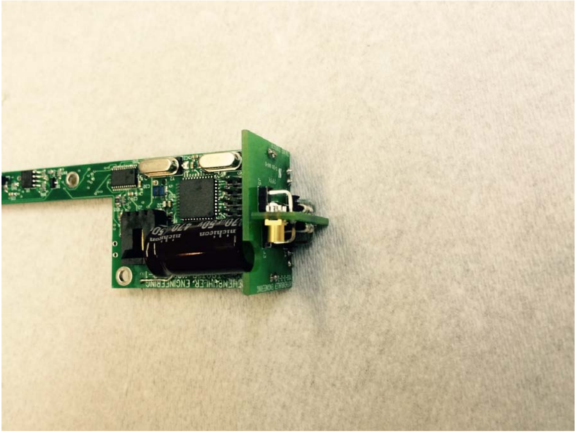
Picture 3 1100-3-2 Digital Board Antenna Interface End View
