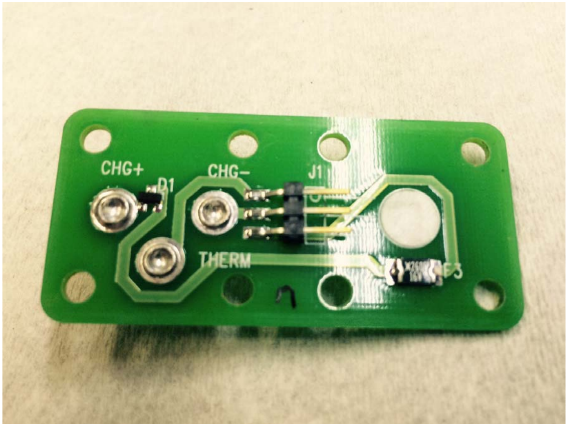
Picture 15 1100-3-2-4 Charge Interface Board Bottom View
