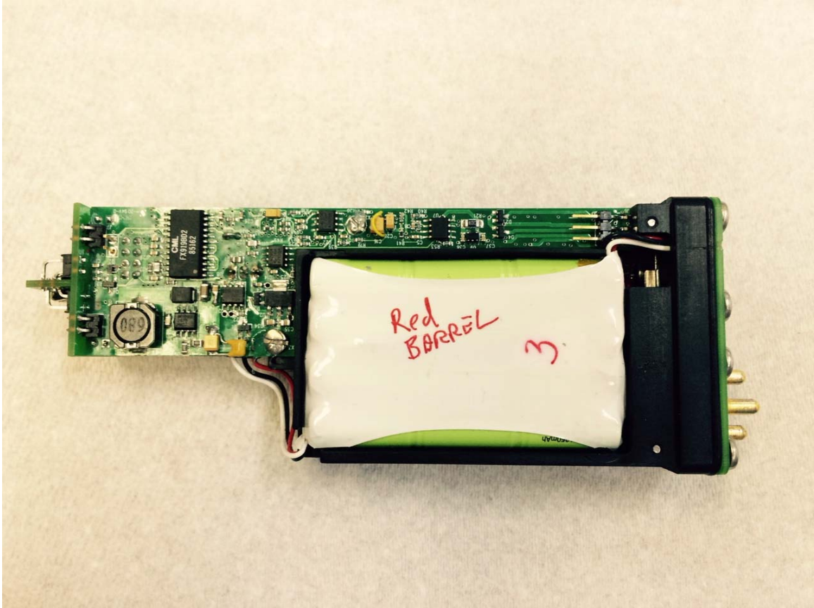
Picture 5 1100-3-2 Internal Assembly Top View
