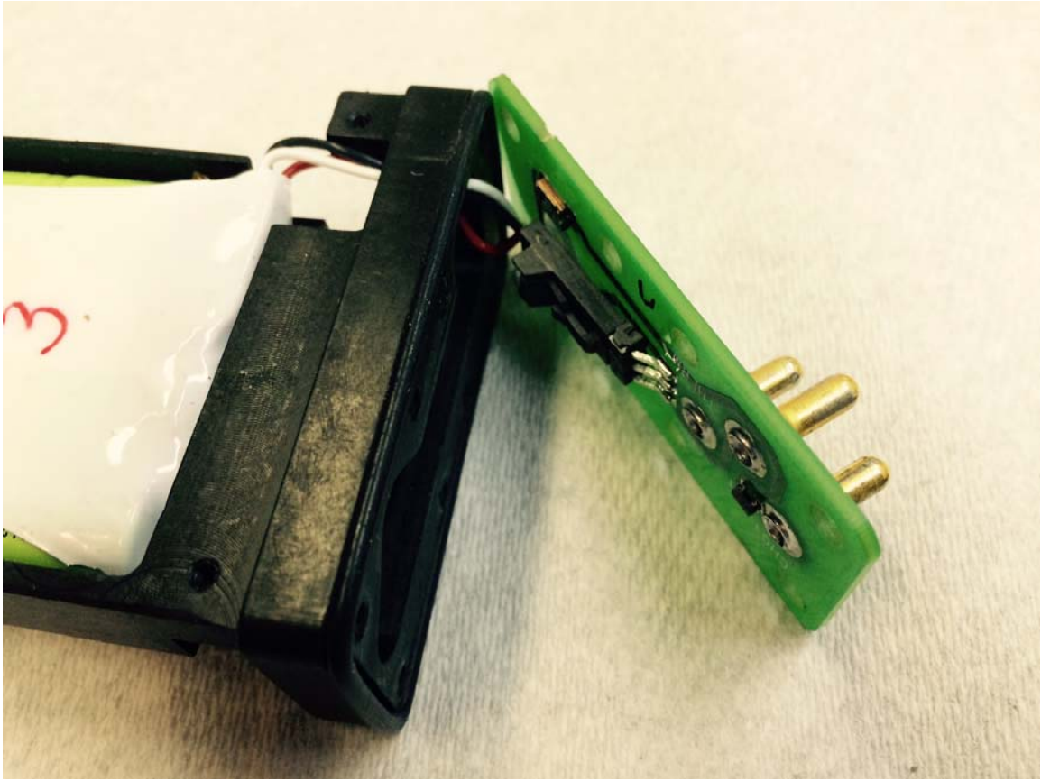
Picture 10 1100-3-2 Internal Interface Battery Block / Charge Board
