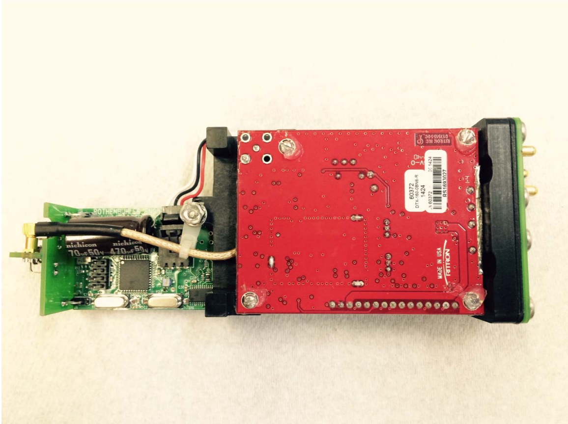
Picture 6 1100-3-2 Internal Assembly Bottom View
