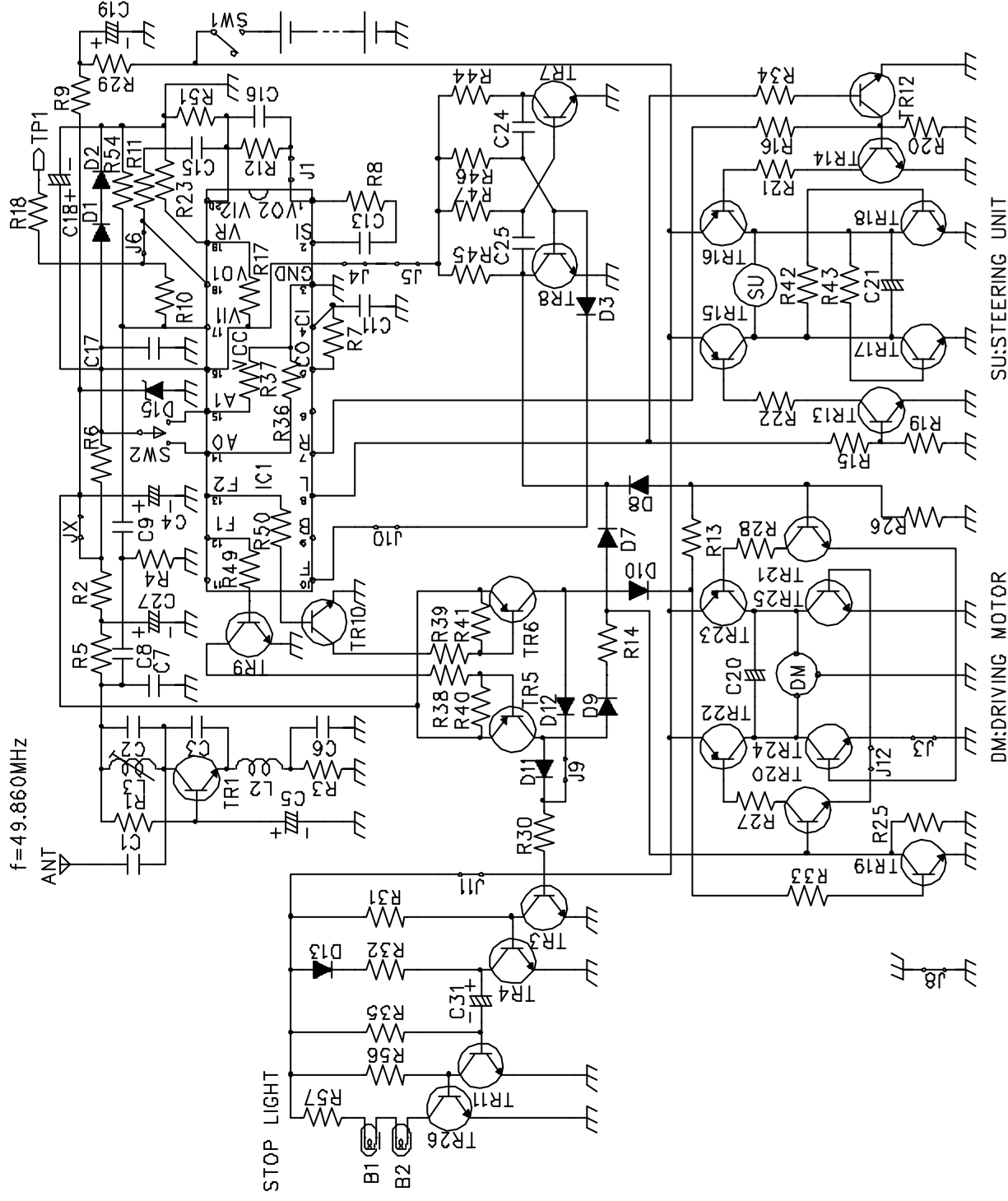
NO.RP6450 CIRCUIT DIAGRAM
