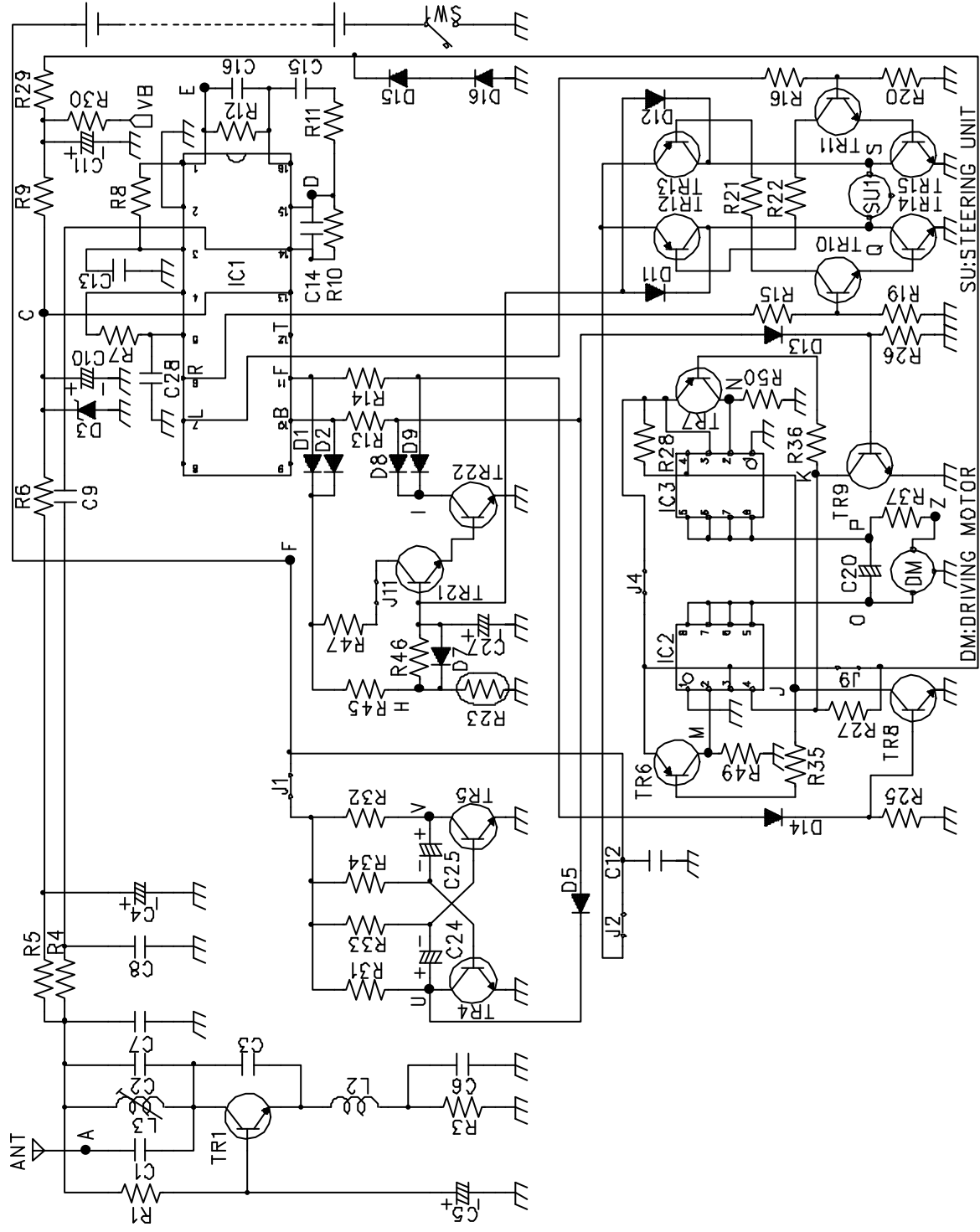
NO.RP6401 CIRCUIT DIAGRAM FCC ID:CVTRP6401H
