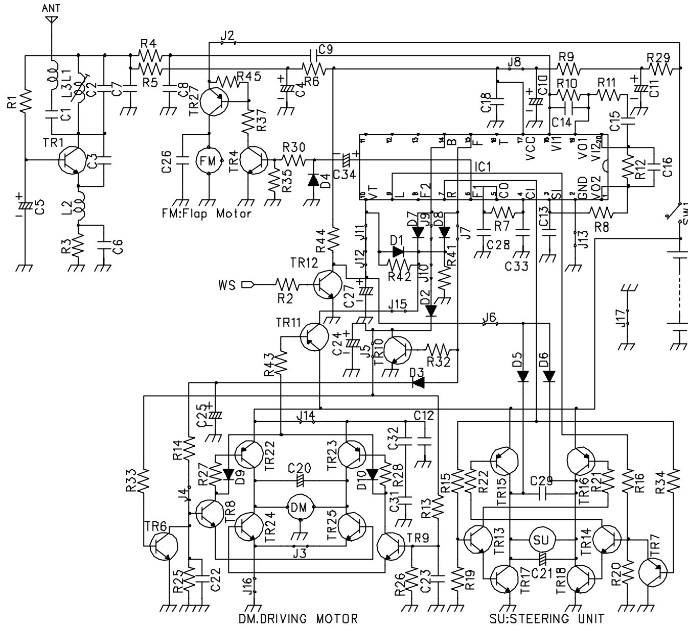
NO.RA4040 CIRCUIT DIAGRAM
