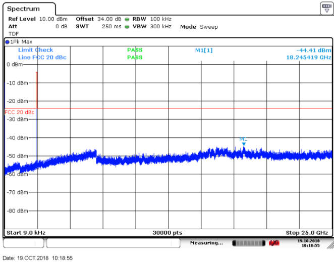
Figure 8.7-3: Conducted spurious emissions outside restricted band, Low channel
