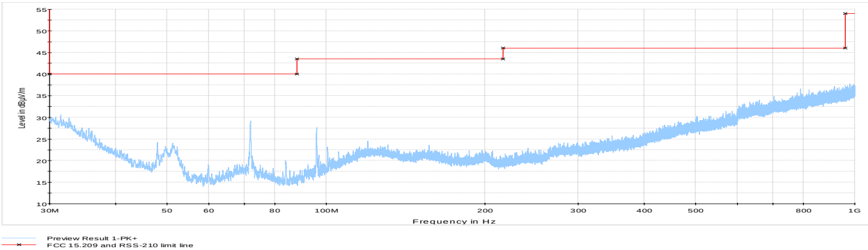
Figure 8.7-7: Radiated spurious emissions 30 MHz to 1 GHz, mid channel
