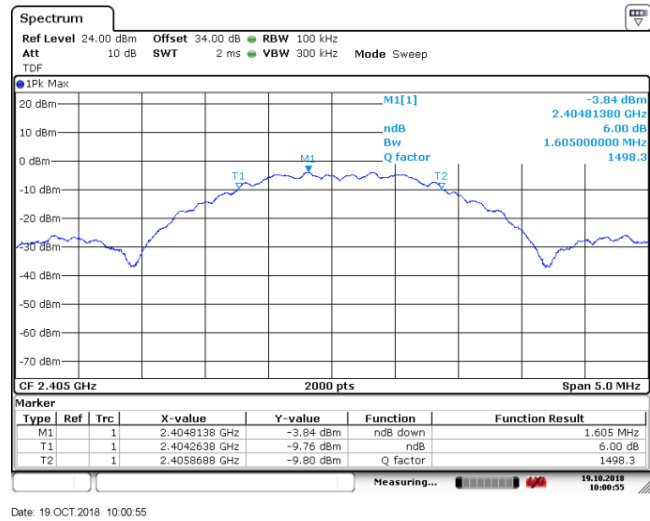
Figure 8.8-1: PSD plot on Low channel
