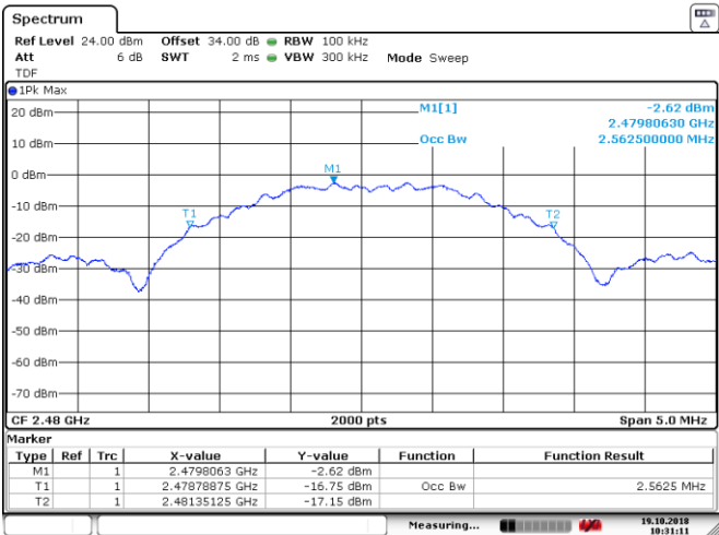
Figure 8.5-6: 99% bandwidth on high channel
