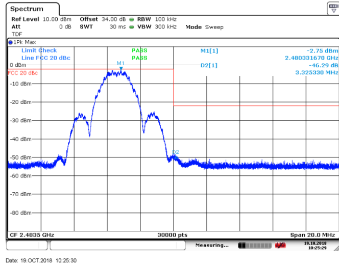
Figure 8.7-2: Conducted spurious emissions at band edge outside restricted band, High channel
