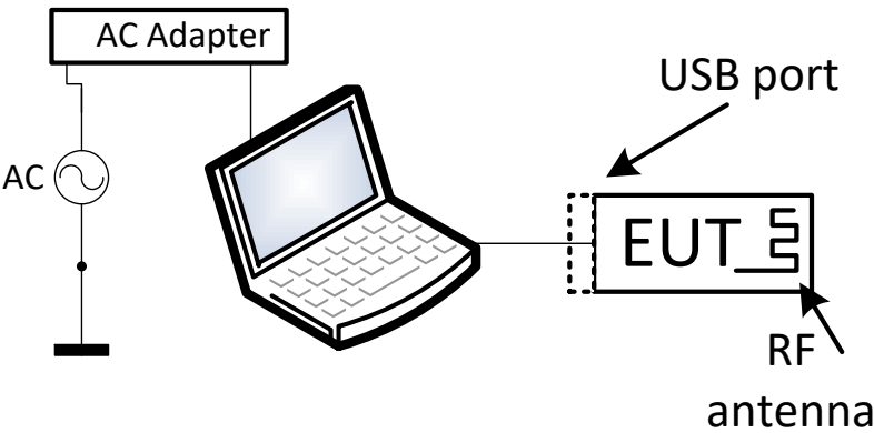
Figure 3.6-1: Setup diagram
