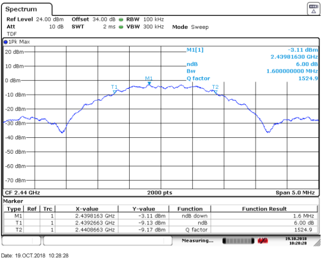
Figure 8.8-2: PSD plot on Mid channel
