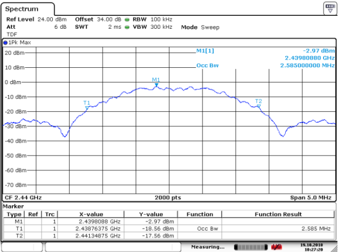
Figure 8.5-5: 99% bandwidth on mid channel
