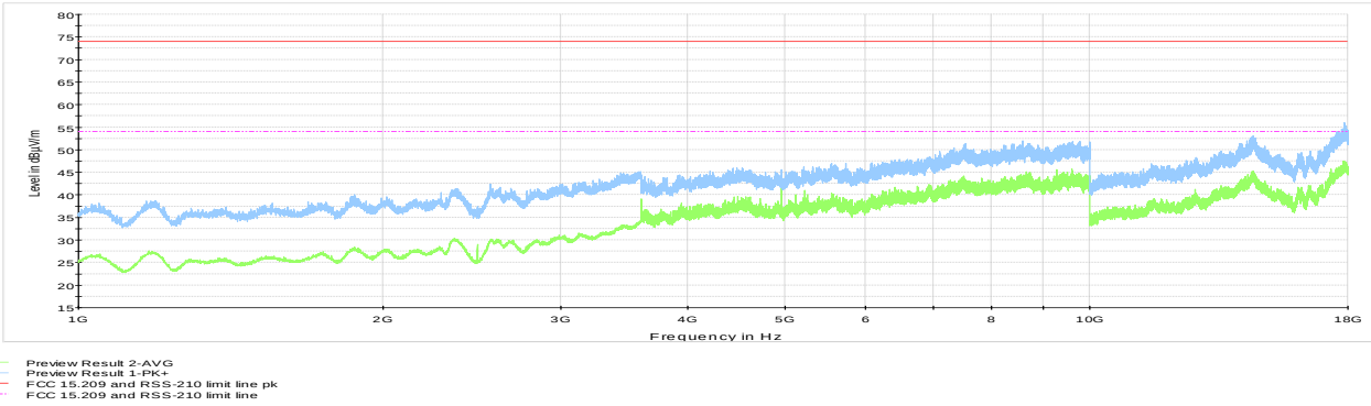
Figure 8.7-11: Radiated spurious emissions 1 to 18 GHz, High channel
