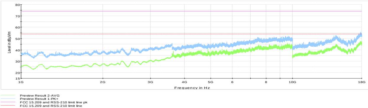
Figure 8.7-10: Radiated spurious emissions 1 to 18 GHz, mid channel
