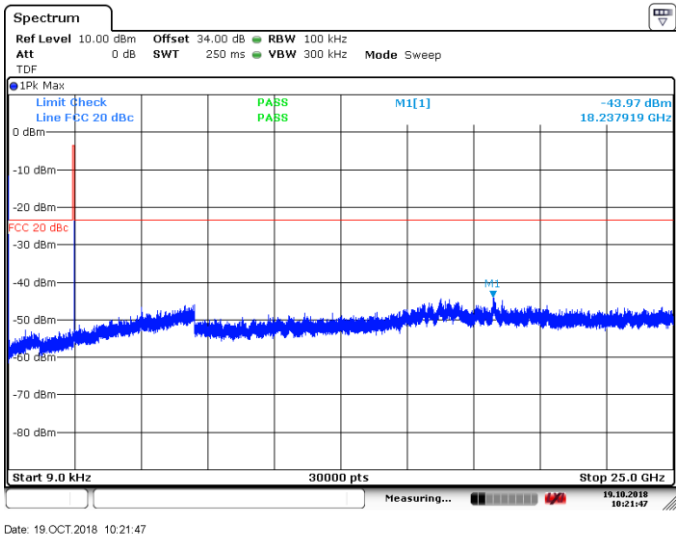
Figure 8.7-5: Conducted spurious emissions outside restricted band, High channel
