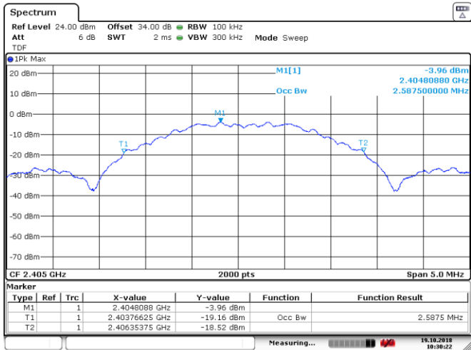
Figure 8.5-4: 99% bandwidth on low channel
