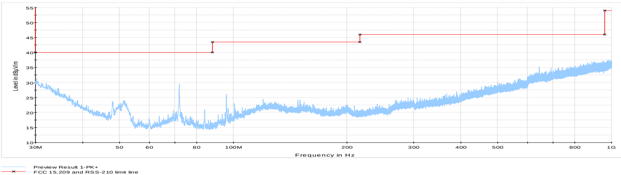
Figure 8.7-8: Radiated spurious emissions 30 MHz to 1 GHz, High channel
