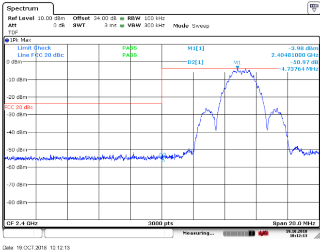
Figure 8.7-1: Conducted spurious emission at band edge outside restricted band, low channel
