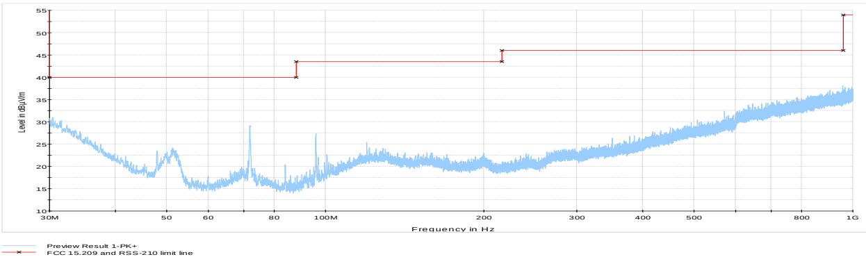
igure 8.7-6: Radiated spurious emissions 30 MHz to 1 GHz, Low channel
