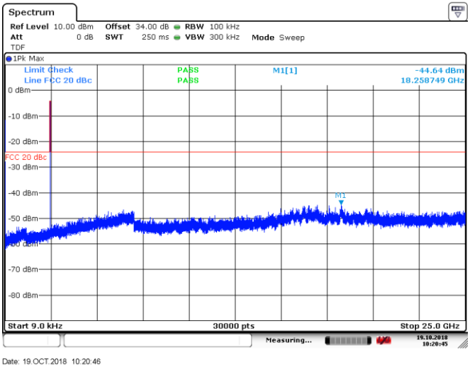
Figure 8.7-4: Conducted spurious emissions outside restricted band, Mid channel
