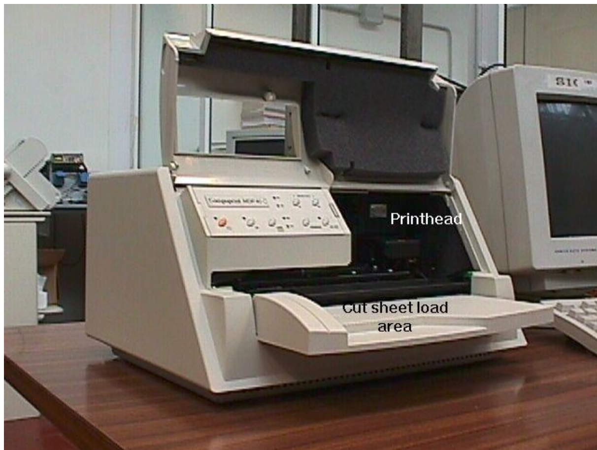
picture 2: front view with the front cover open
