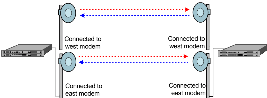
Figure 2-10. 1+1 Protection in Diversity Mode
