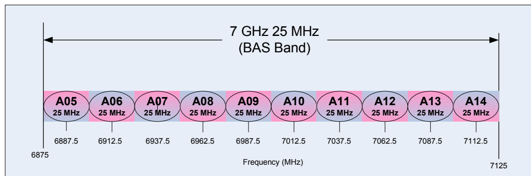
Figure 3-6. 7 GHz, 25 MHz BAS Frequency Plan
