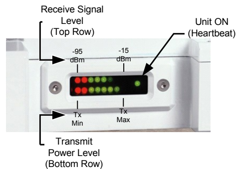
Figure 2-4. ODU 2200 RSSI Output vs. Received Signal.
