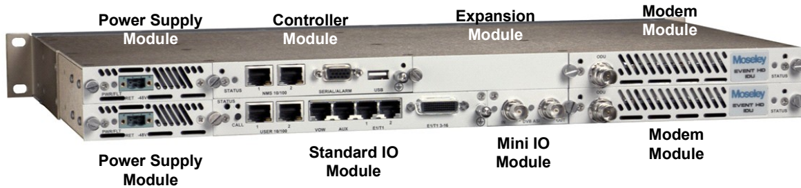
Figure 3-22. SDIDU™ Modules
