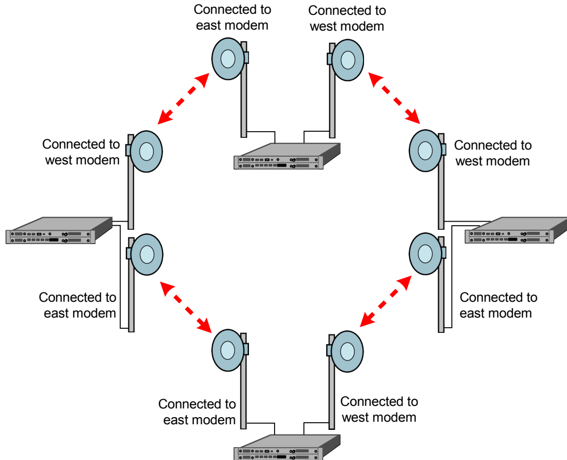
Figure 2-8. 2 + 0 (East West) Configuration
