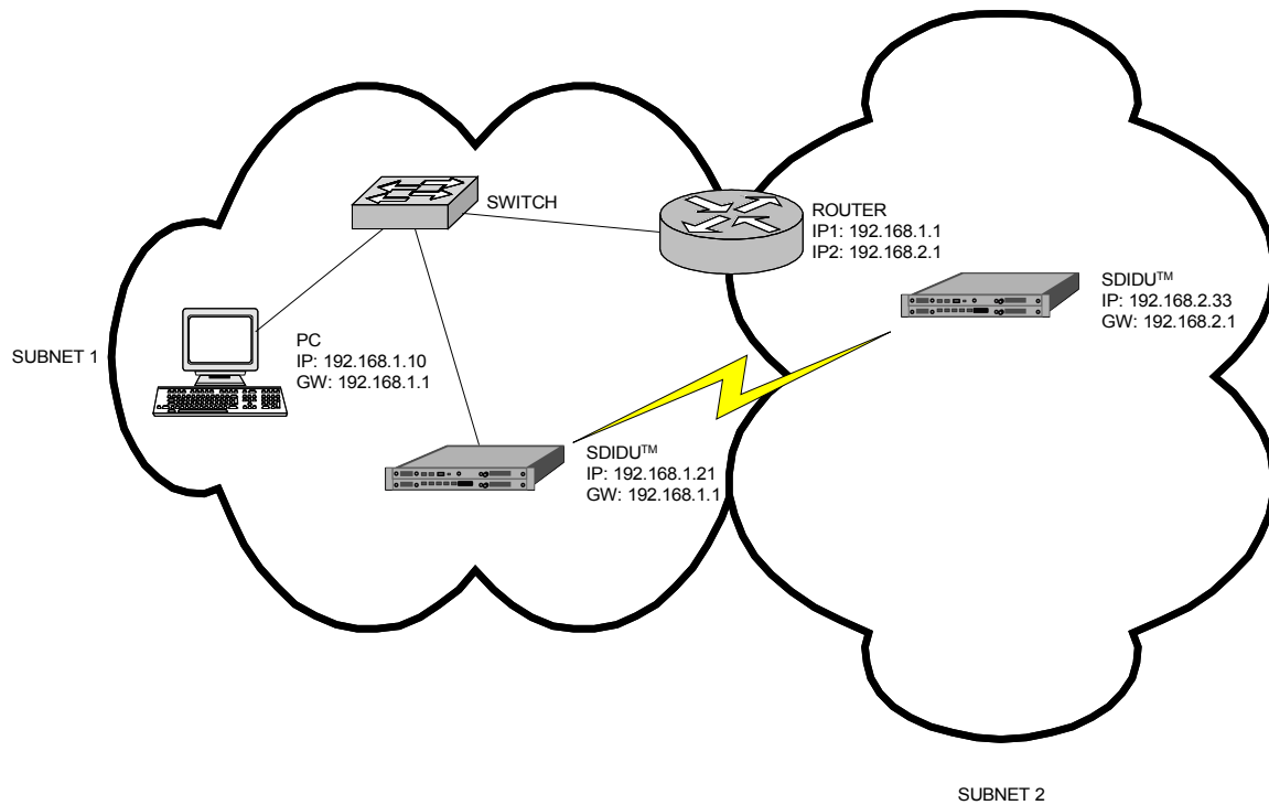
Figure 2-15. Event-HD SDIDUs™ on Different Subnets
