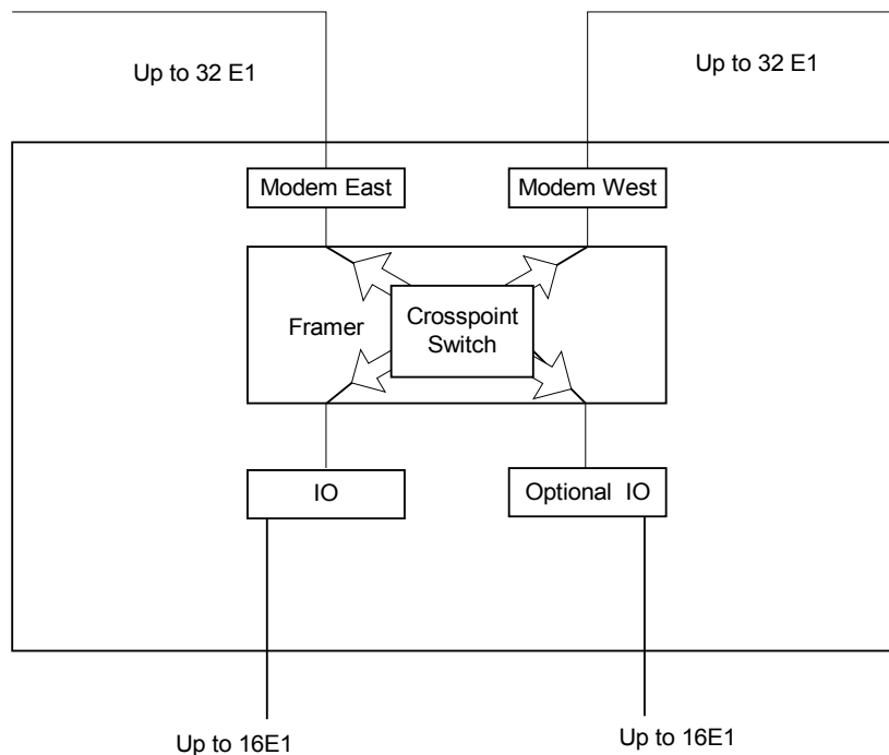
Figure 2-12. Crosspoint Switch
