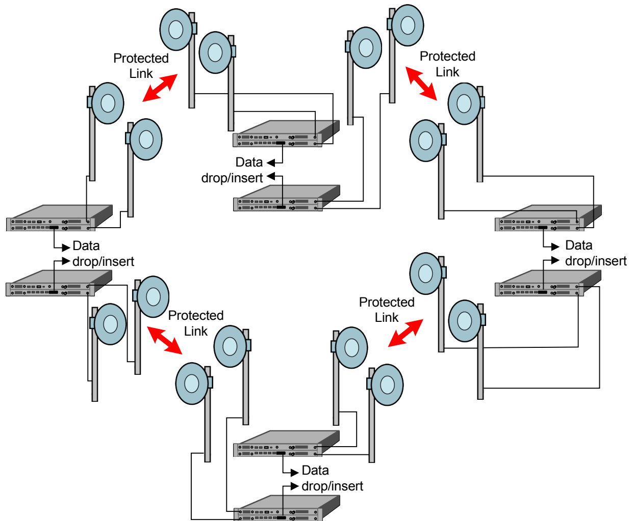
Figure 2-11. 1 + 1 Multi-Hop Repeater Configuration
