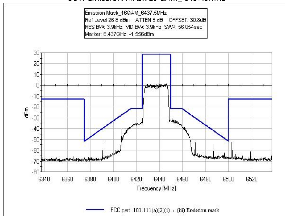
OBW EMISSION MASK 16 QAM_6437.5MHz
