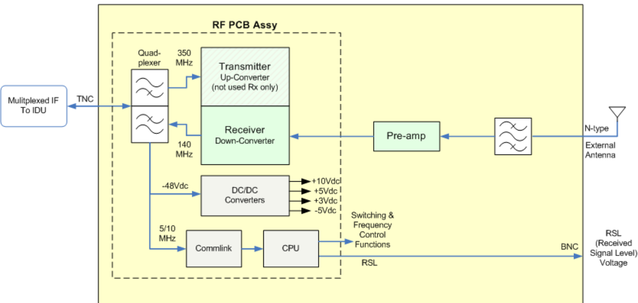
ODU Assy
