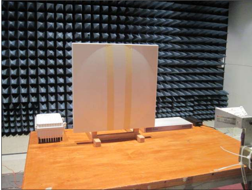
Photograph 7. Radiated Spurious Emissions, Test Setup, 18 GHz – 26 GHz
