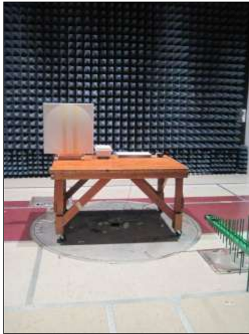
Photograph 3. Radiated Emission, Test Setup, 30 MHz – 1 GHz
