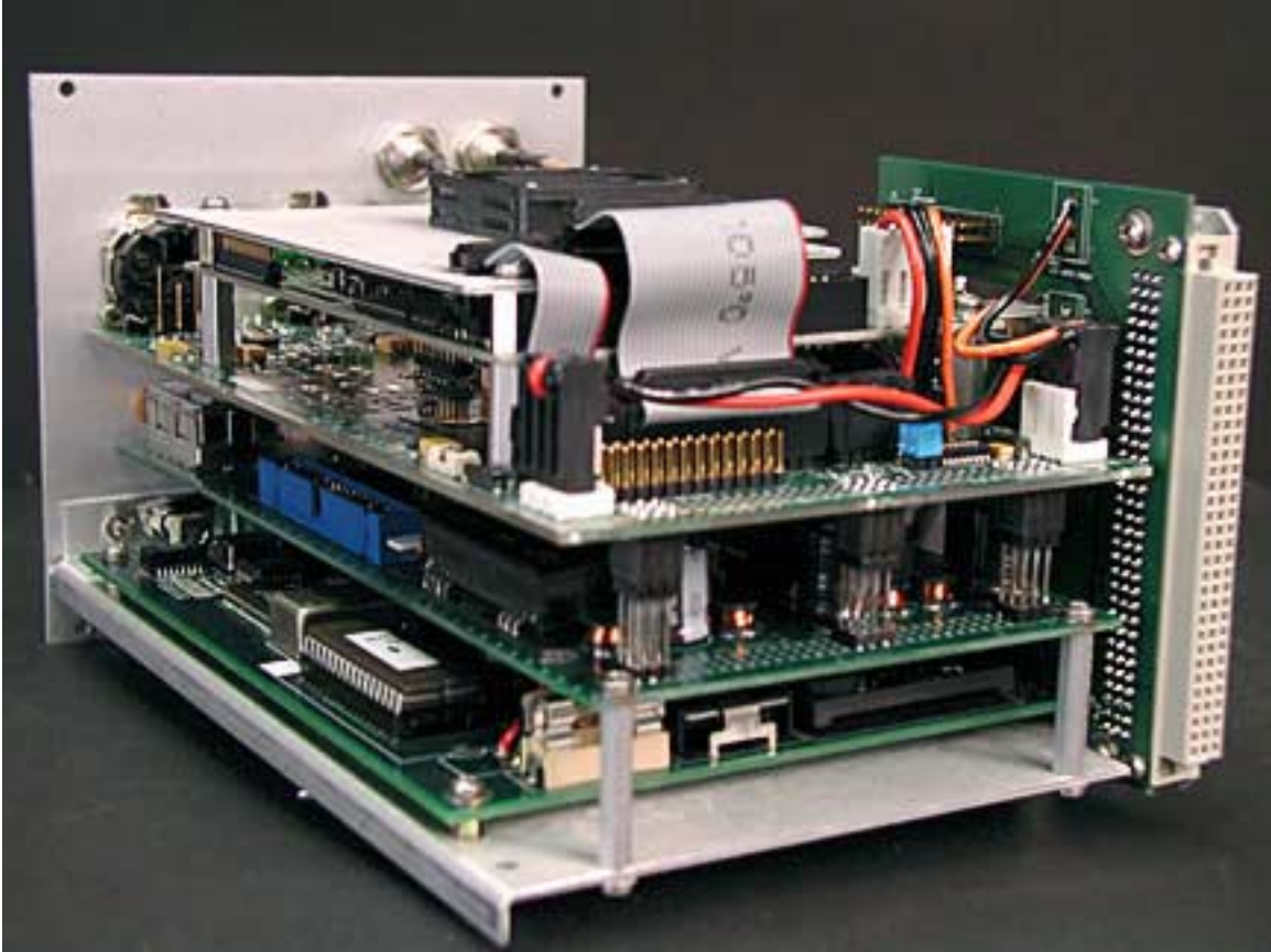
MpegEnc COFDMMod Rear Angle 1
