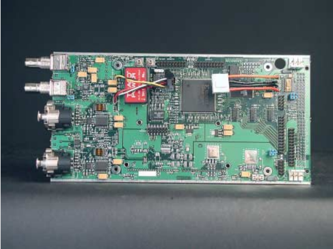
930-13565-12ENC-BBC-PVR Controller
