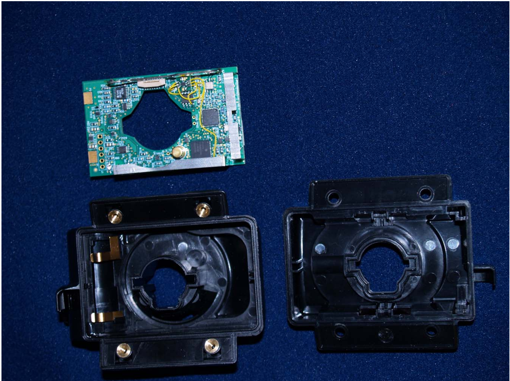
Photo 2: TAD (TAD-001) – Case halves opened w/PCB removed
