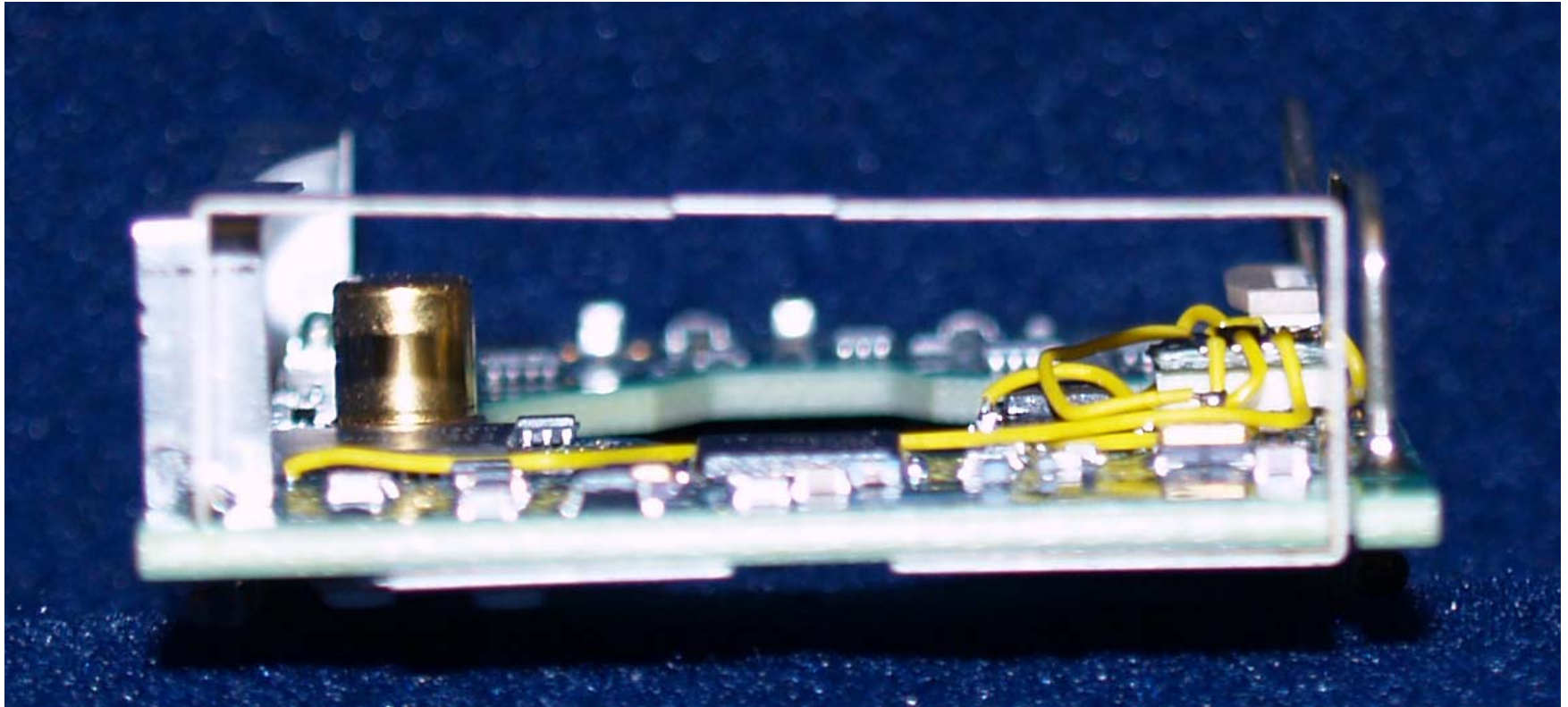
Photo 6: TAD (TAD-001) – PCB (end view)
