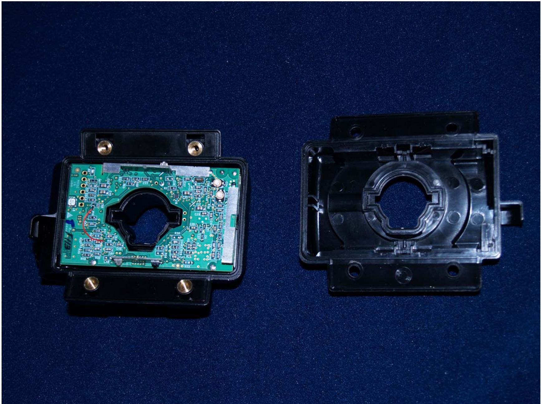
Photo 1: TAD (TAD-001) – Case halves-opened
