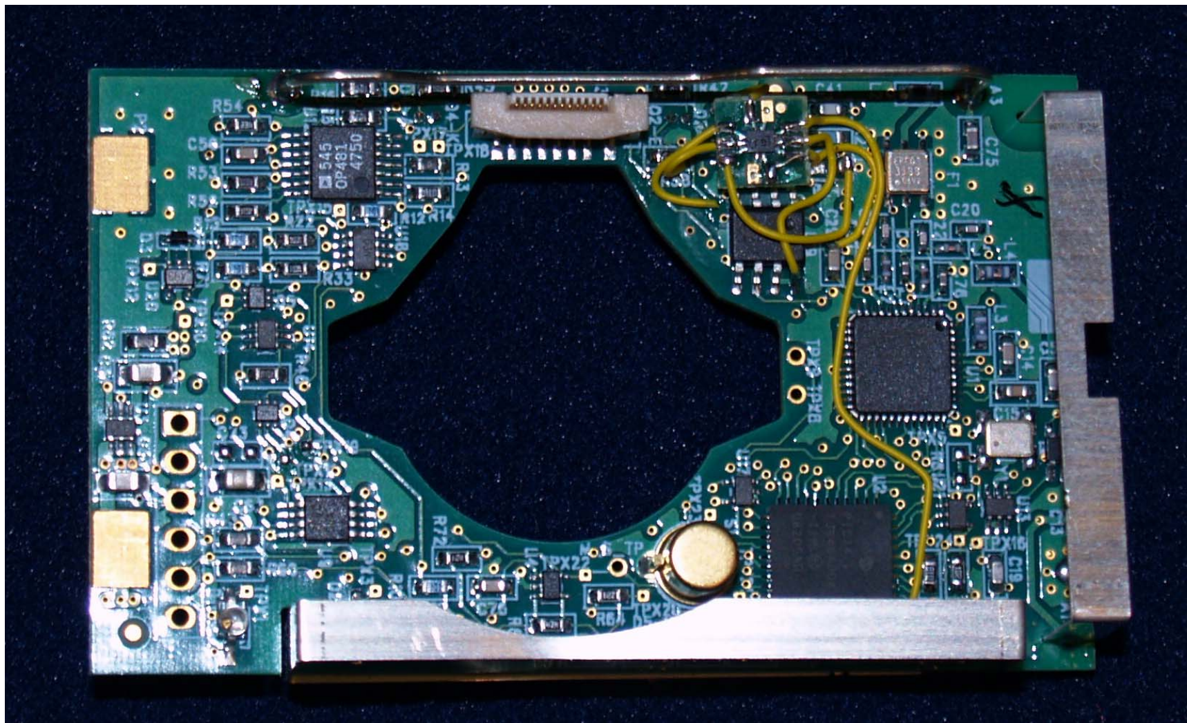
Photo 4: TAD (TAD-001) – PCB (top side)
