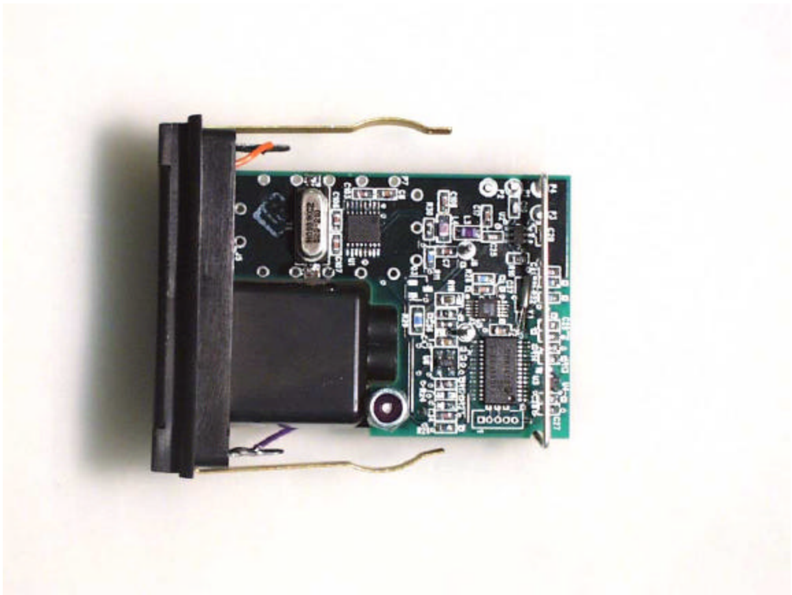
PCB WITHOUT ANTENNA
