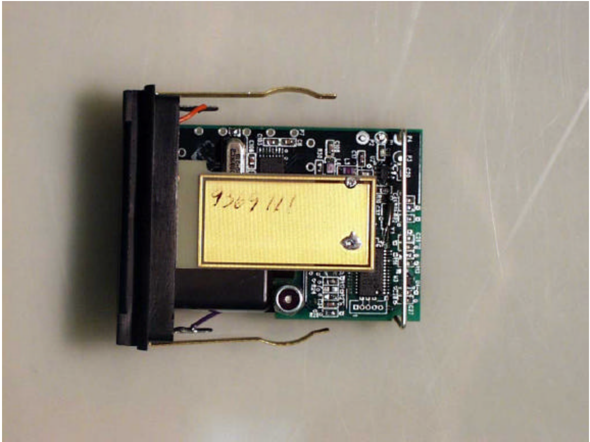
PCB ANTENNA MOUNTED
