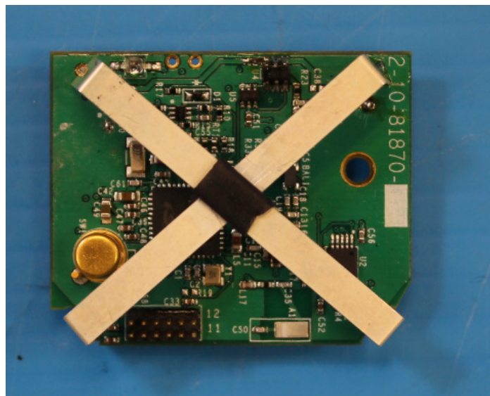
Pic 2 – BI HomeGuard 20\20 Transmitter board Top Side with antenna installed
