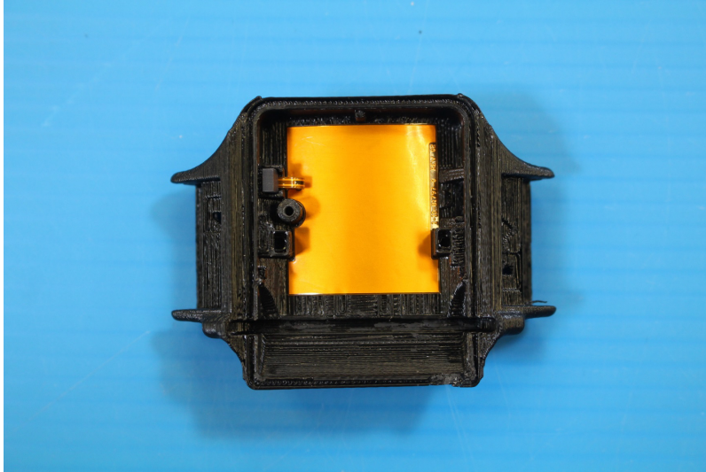
Pic 5 – HomeGuard 20/20 Transmitter - Proximity Flex installed
