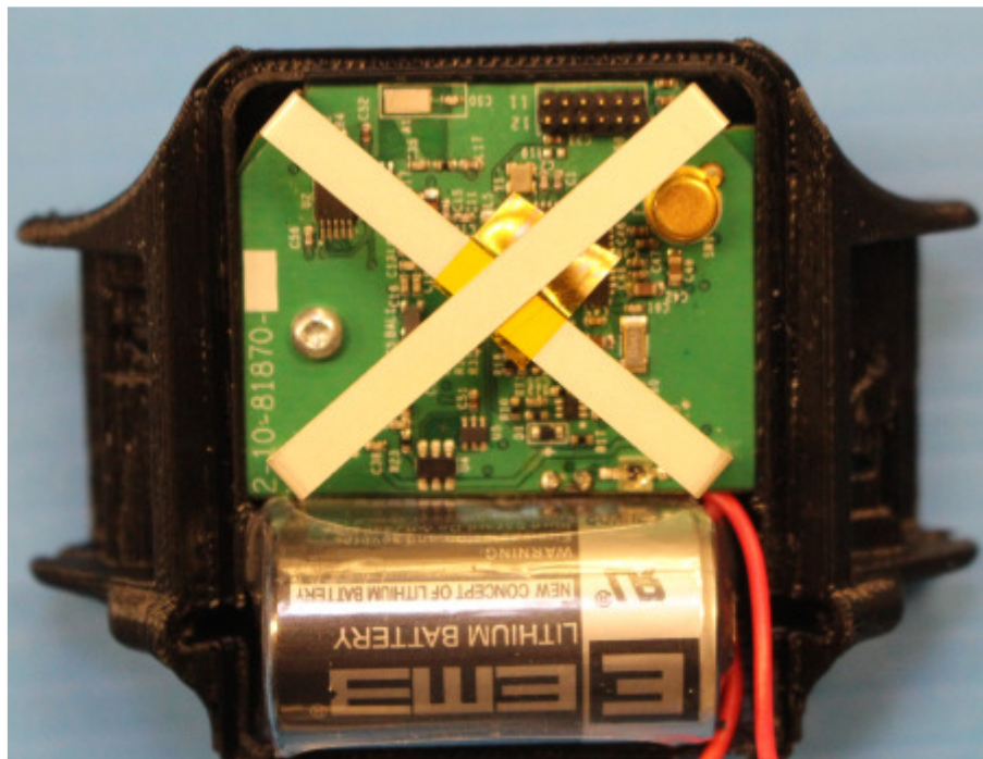
Pic 6 - HomeGuard 20/20 Transmitter – in housing
