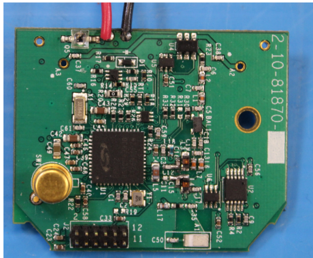
Pic 1 – BI HomeGuard 20\20 Transmitter board Top Side
