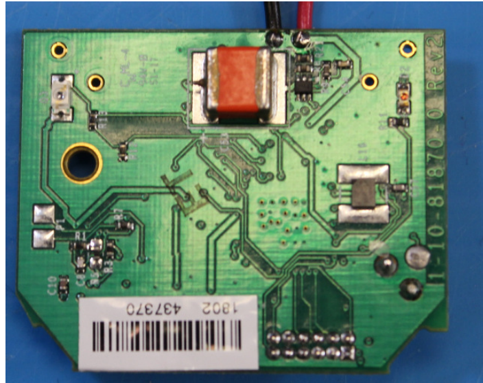
Pic 3 – BI HomeGuard 20/20 Transmitter board bottom Side
