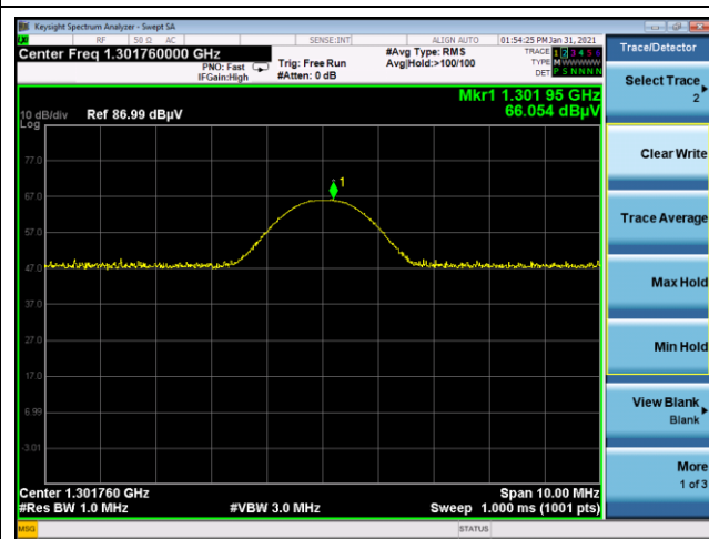
5 th harmonic
