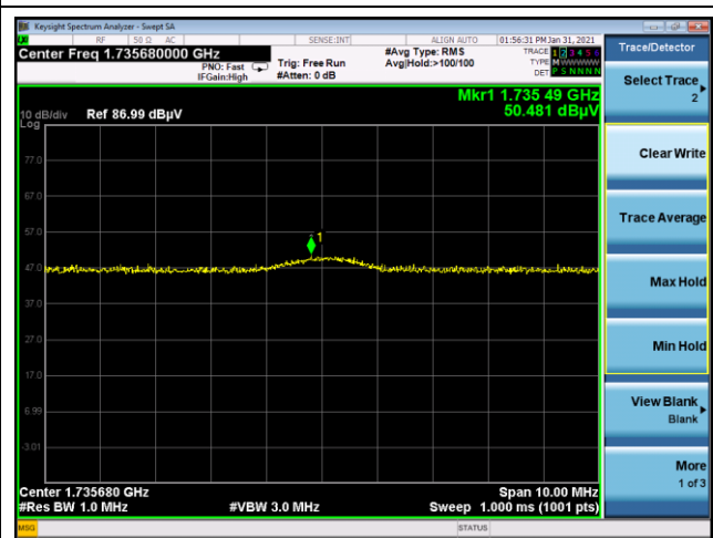
6 th harmonic
