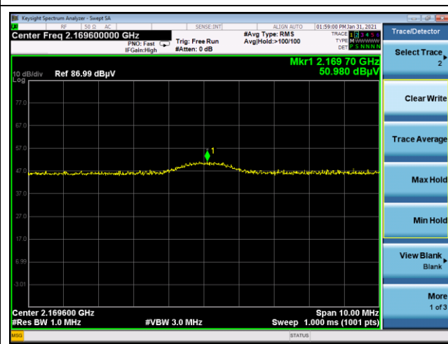
5 th harmonic
