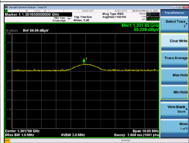
5 th harmonic
