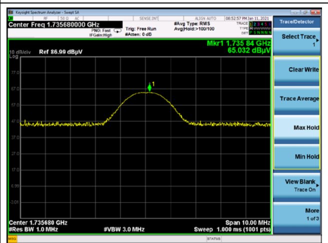
8 th harmonic
