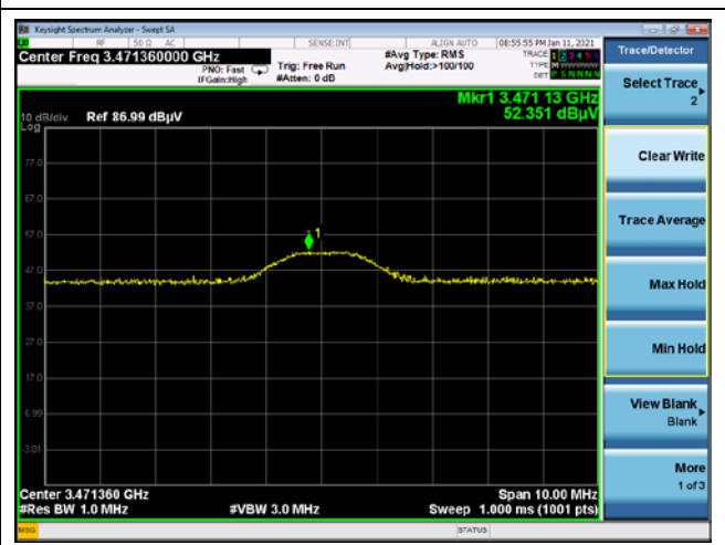
8 th harmonic
