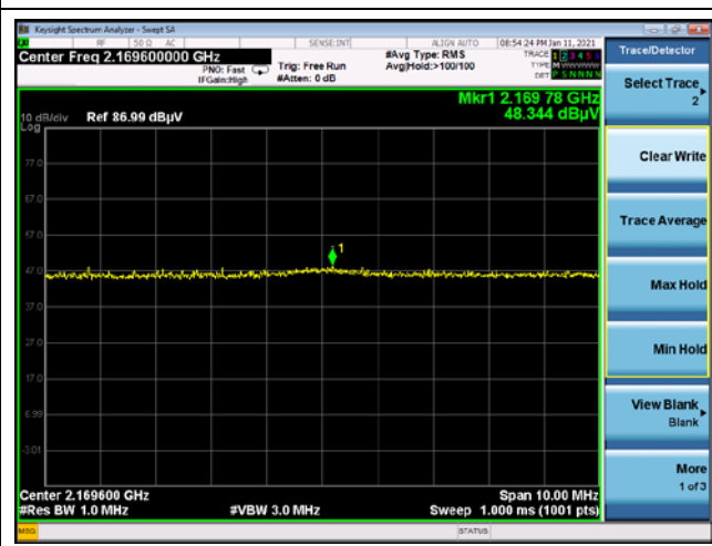
5 th harmonic
