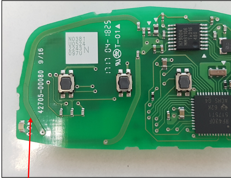
PCB Antenna
