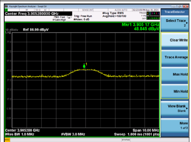
9 th harmonic
