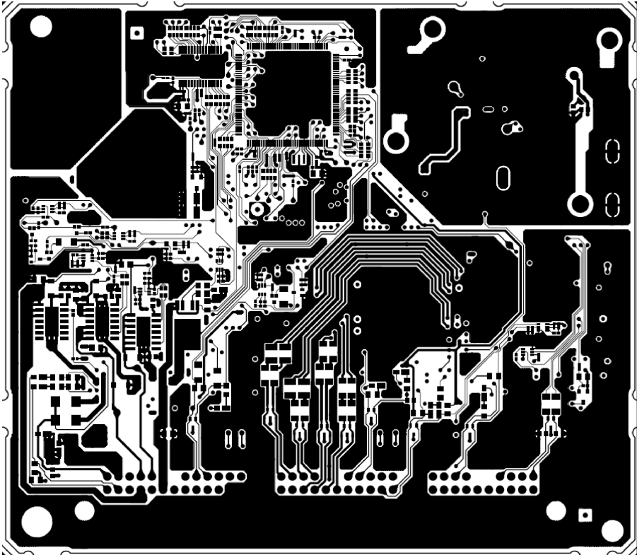
Solder Side
