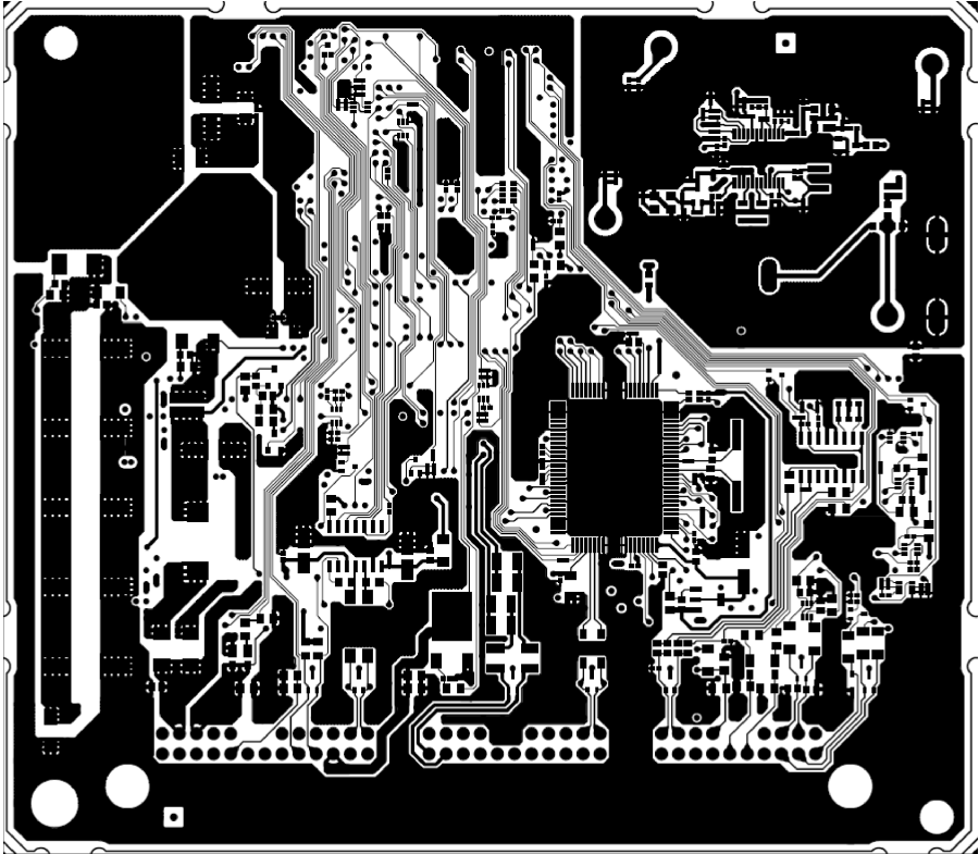
Component Side
