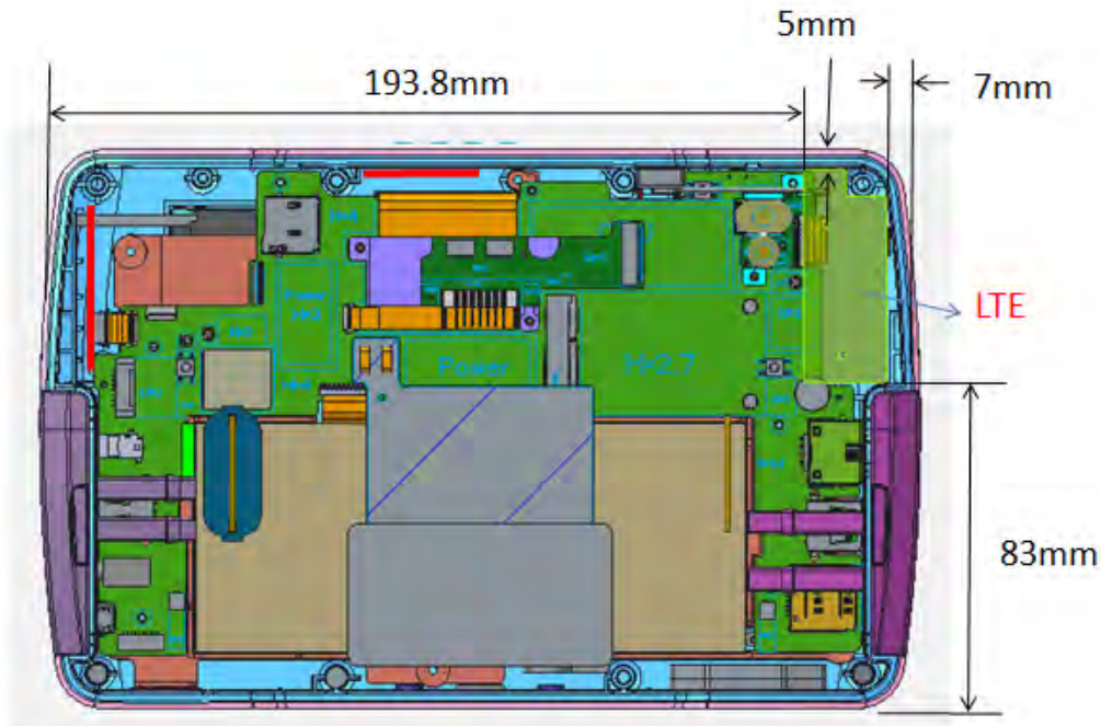
Fig.14 Antenna separation distance of EUT (WWAN antenna)
