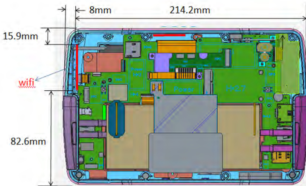
Fig.15 Antenna separation distance of EUT (WLAN Main/BT antenna)
