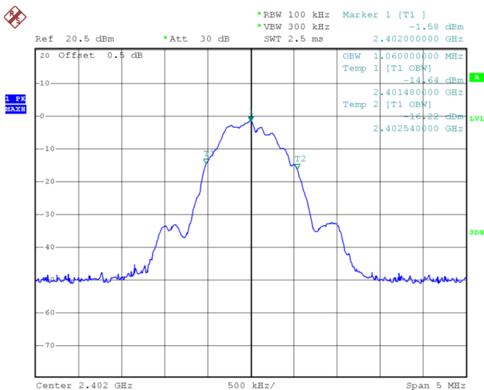
(Plot A2:Channel 0: 2402MHz)
