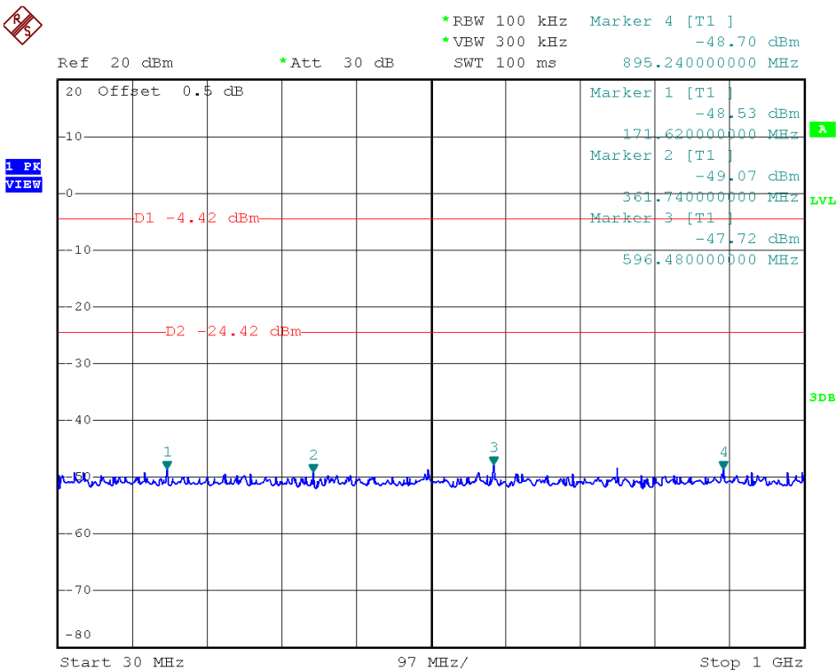
(Plot H.1: Channel = 39, 30MHz to 1GHz @ 8-DPSK)
