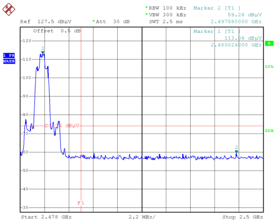
(Plot F1: Channel = 78 PEAK @ 8-DPSK Mode)
