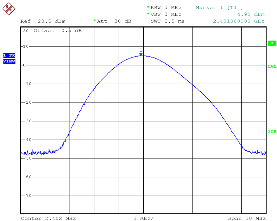
Plot C1:8-DPSK
