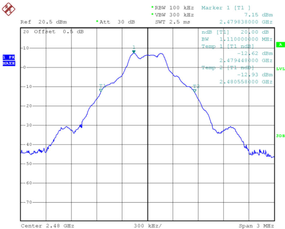
(Plot C: Channel = 2480 @ GFSK)
