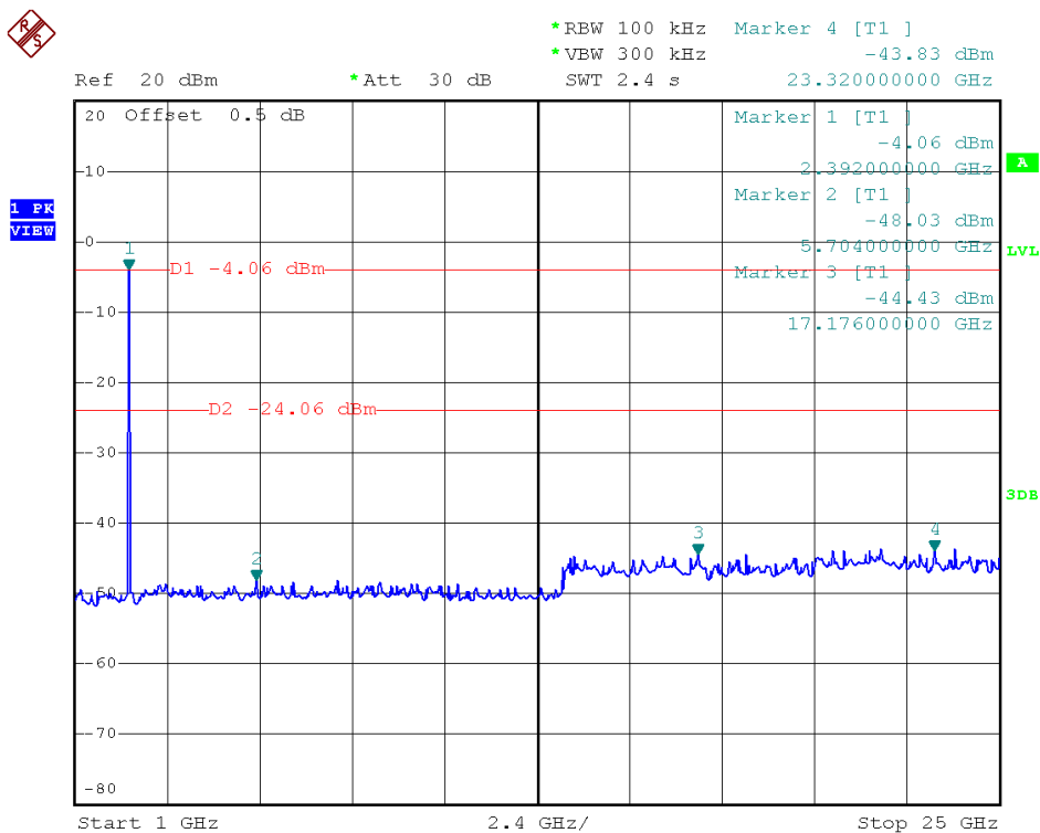
(Plot D.2: Channel = 0, 1GHz to 25GHz @ \pi/4 -DQPSK)
