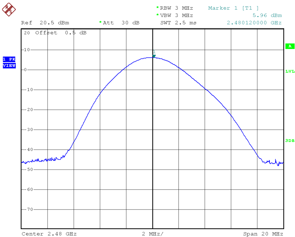
Plot A2: GFSK
