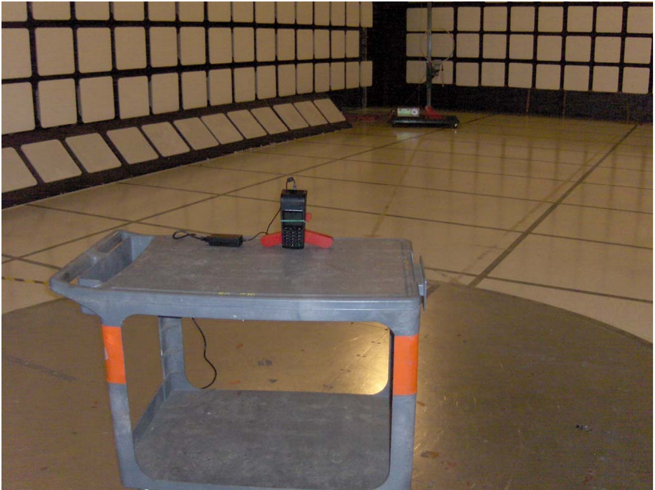
Radiated Emissions @ 10 m – Orthogonal Position 3
