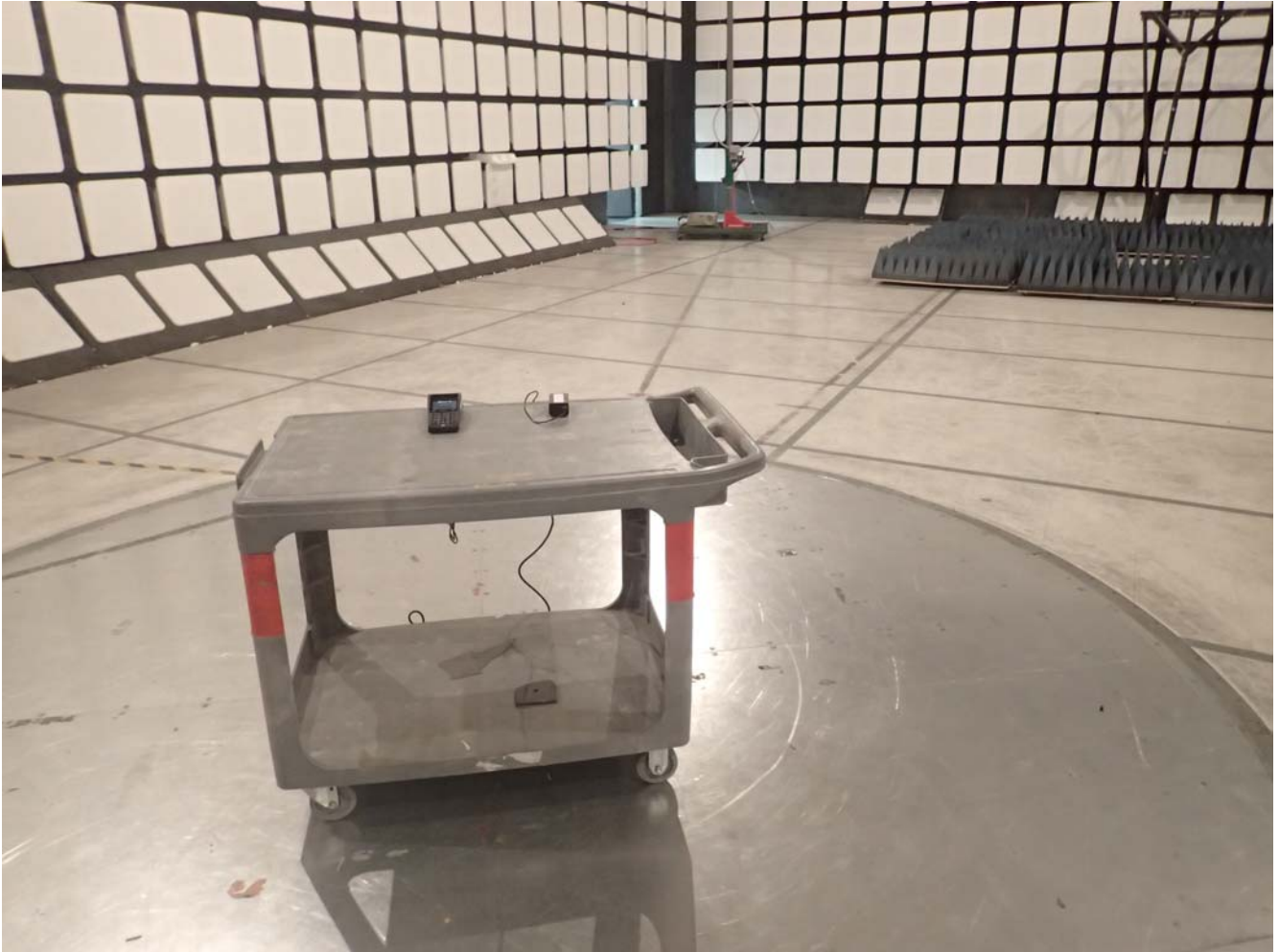
Radiated Emissions @ 10 m – Orthogonal Position 1
