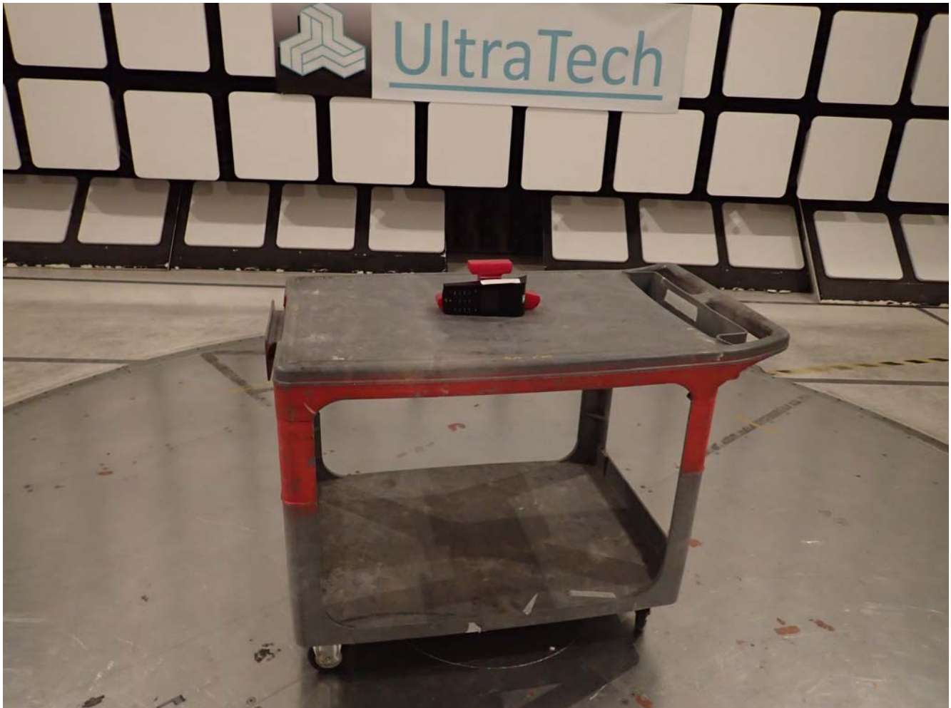
Radiated Emissions @ 3 m/10 m – Orthogonal Position 2
